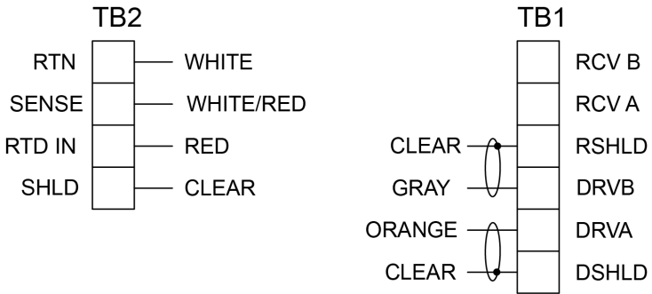
Figure 2-11: Wiring for Rosemount 1066 transmitter
