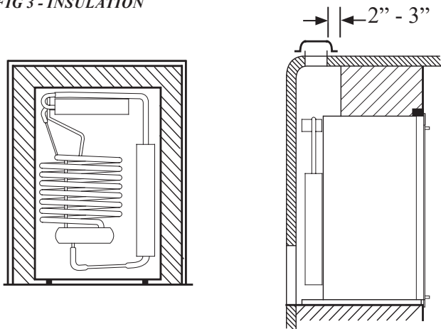
FIG 3 - INSULATION
