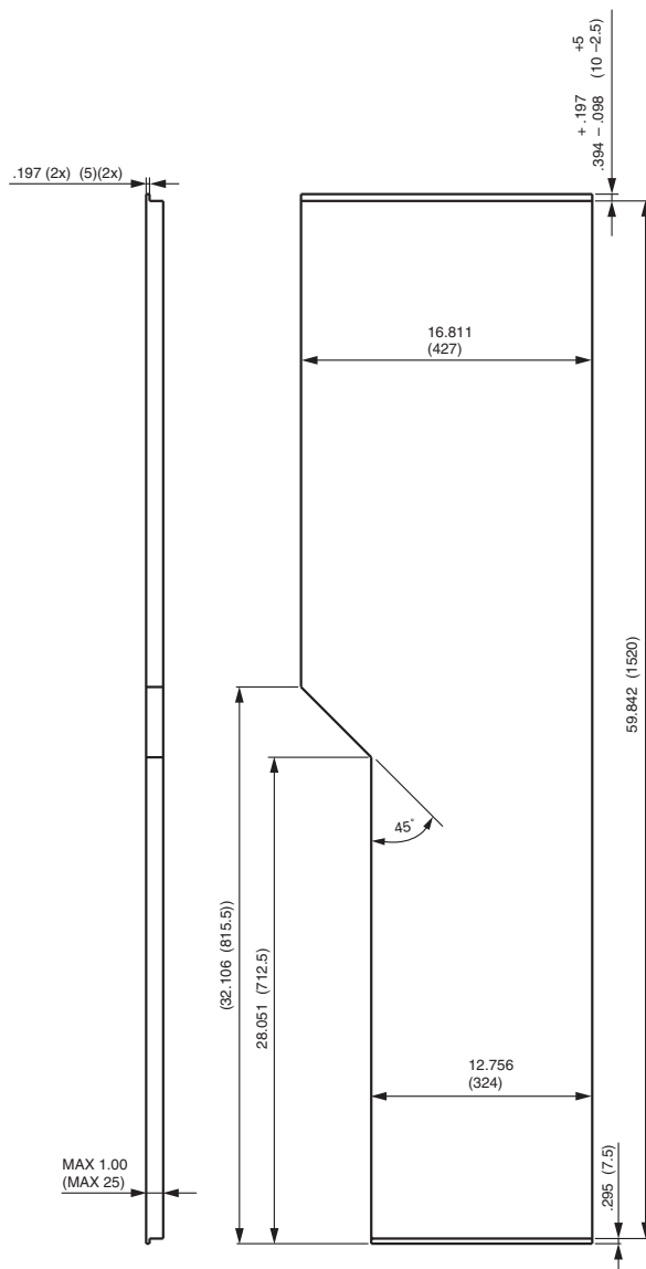
FIG24-PANEL DIMENSIONS FOR THE FRIDGE DOOR
