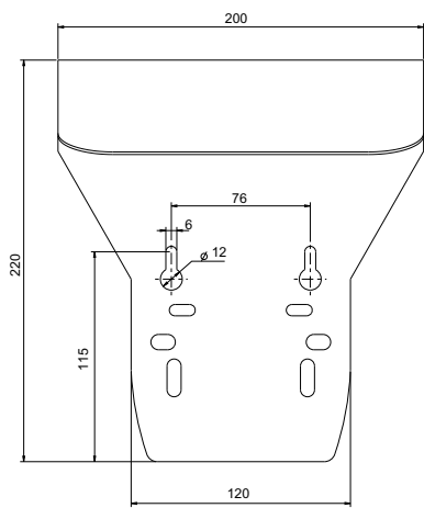
Fig. 28 Dimensions sunshield
