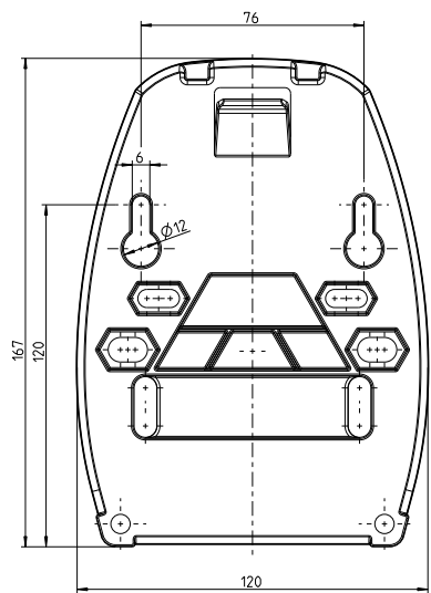
Fig. 27 Installation mounting plate
