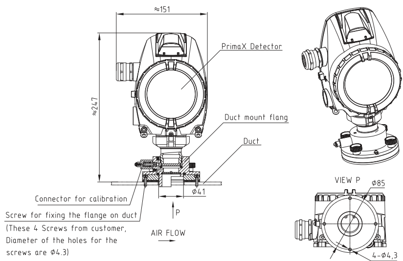
Fig. 29 Duct mounting
