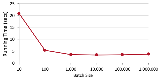
Figure 15: The effect of different batch sizes on the performance of FFT with tumbling windows
