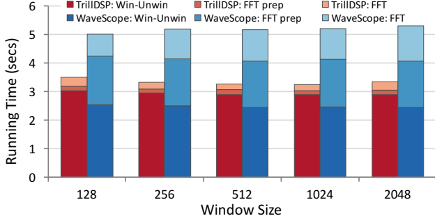
Figure 13: Cost breakdown of FFT with tumbling window
