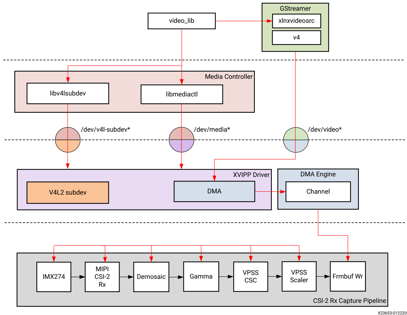
Figure 5: VL42 Driver Stack
