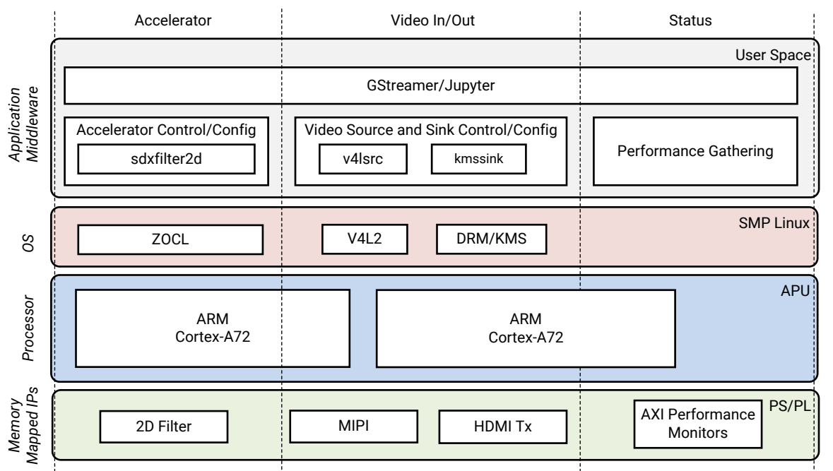
Figure 2: Key Reference Design Components by Processing Unit
