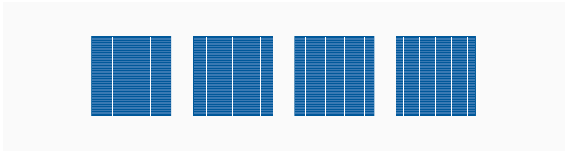
Figure 13 from left to right: 2BB 6" polycrystalline solar cell; 3BB 6" polycrystalline solar cell; 4BB 6" polycrystalline solar cell; 5BB 6" polycrystalline solar cell
