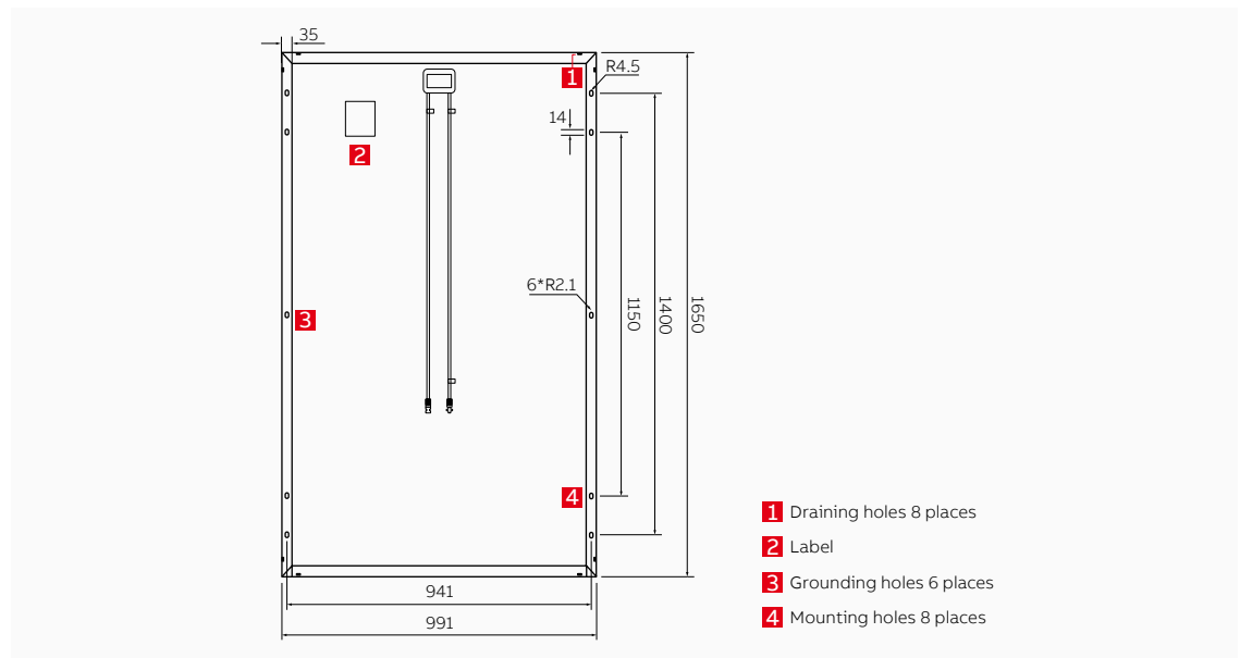
Figure 98 Dimensions of the selected module type
