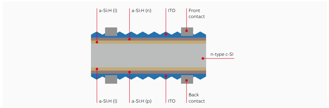
Figure 17 HJT cell stratigraphy; source meyerburger.com
