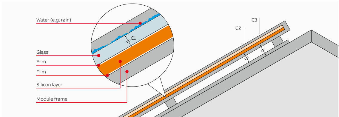
Figure 72 parasitic capacitances
