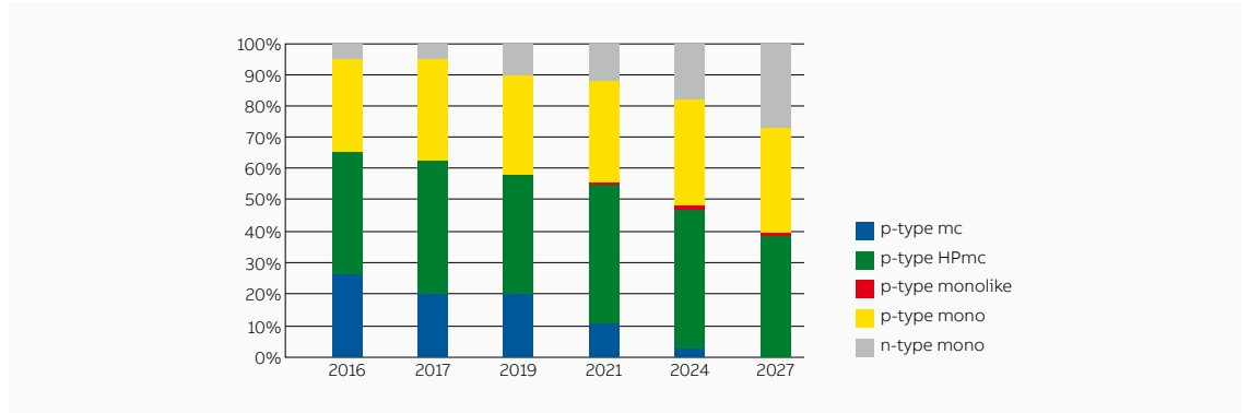
Figure 16 source International Technology Roadmap for Photovoltaic Results 2017
