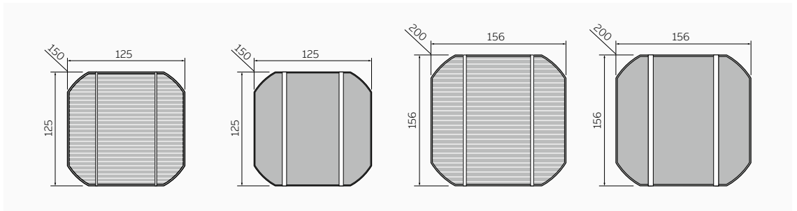
Figure 11 in the left side a 5" semi-square monocrystalline solar cell; in the right side a 6" semi-square monocrystalline solar cell
