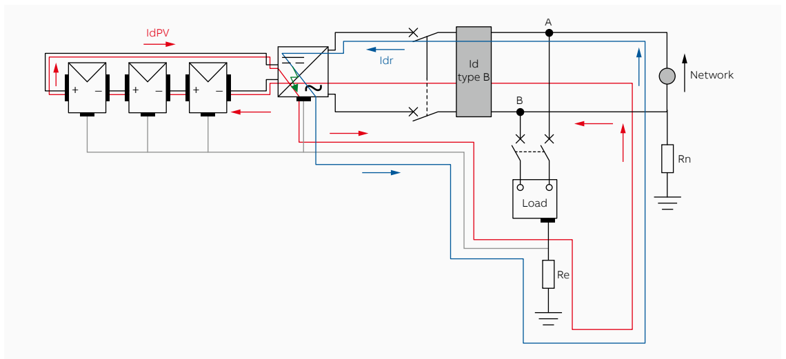
Figure 71 plants with an isolated PV generator, and an inverter transformer-less
