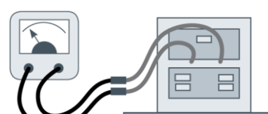
5. Filament winding between terminals, less than 1 \Omega .
