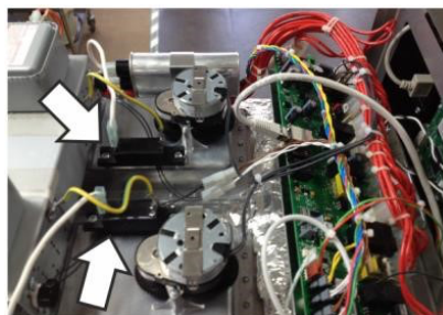
Two high voltage diodes (2000W e2s variant)
