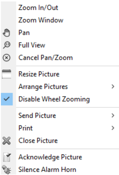
Right-Click Menu
