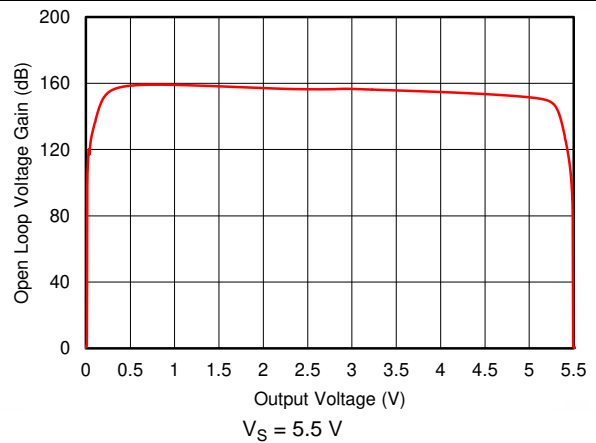
Figure 30. Open Loop Voltage Gain vs Output Voltage
