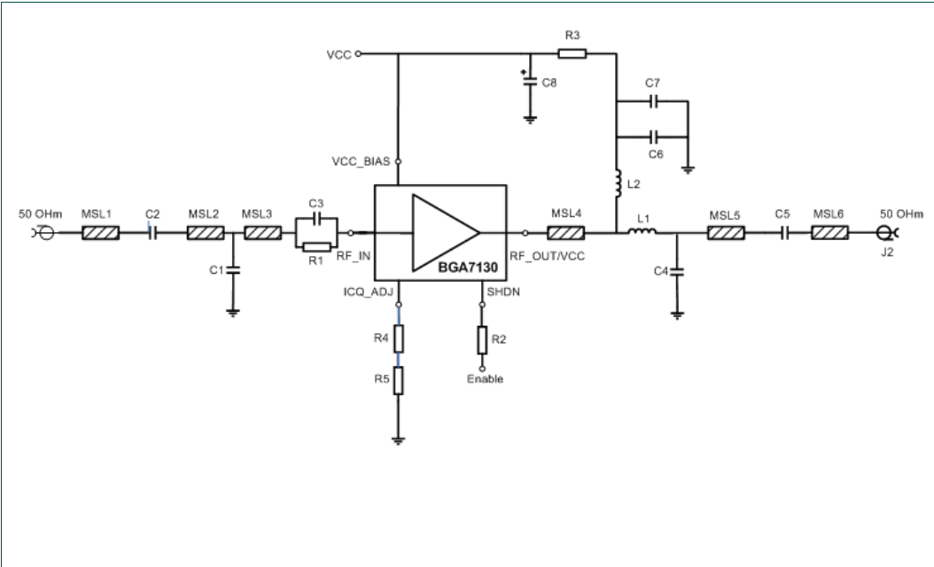
Fig 3. BGA7130 865 - 880 MHz EVB circuit diagram
