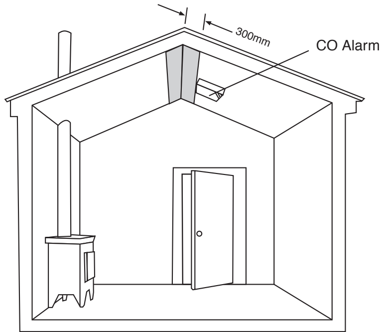
Figure 2. Location in rooms with sloped ceilings
