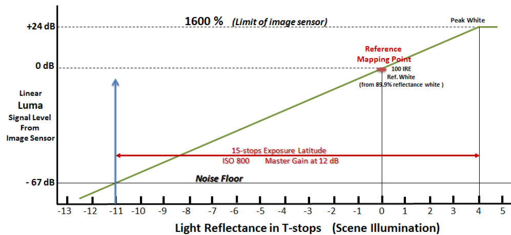
Figure 17 The readjusted camera system mapping of the reference white setting (with Master Gain now set at +12 dB) produces the linear light transfer characteristic as shown
