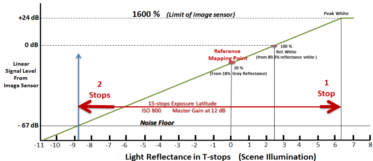
Figure 19 The linear light representation of the S35mm CMOS image sensor with the two arrows indicating the extension of its dynamic range beyond the 12-stop range of the original EOS C300 cine camera
