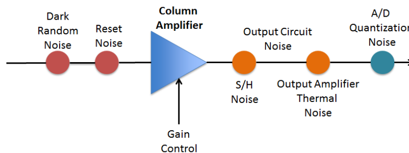
Figure 9 The various noise sources within the CMOS image sensor system
