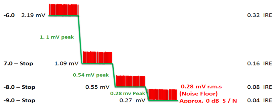
Figure 20 Illustrating the lower video signal levels (in millivolts) and the rms noise associated with the camera Luma specification of 68 dB that define the lower boundary to effective camera dynamic range
