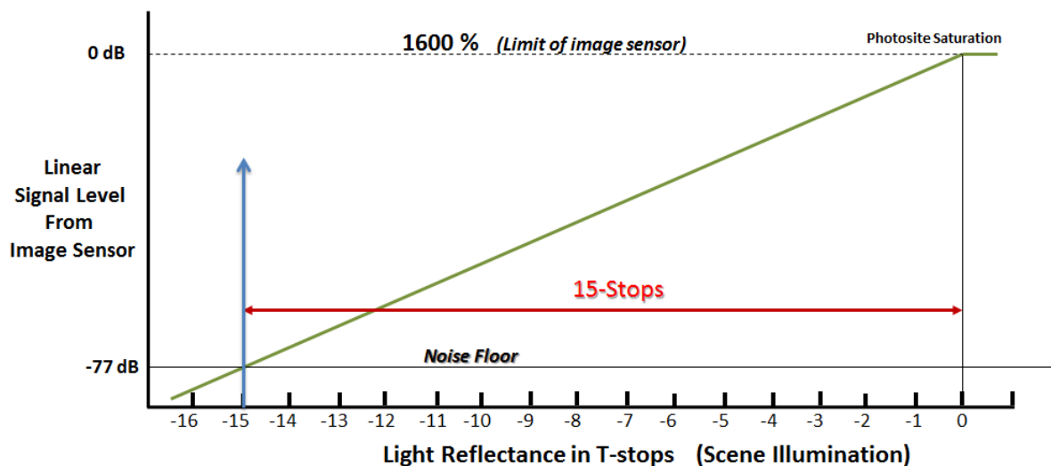
Figure 7 Showing the 15-Stop linear light transfer characteristic of the CMOS image sensor in the EOS C700 and EOS C300 Mark II cameras
