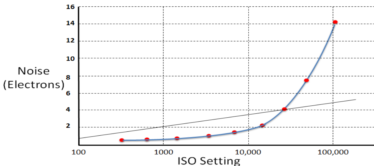
Figure 11 The behavior of EOS C300 Mark II image sensor noise over the range of ISO settings
