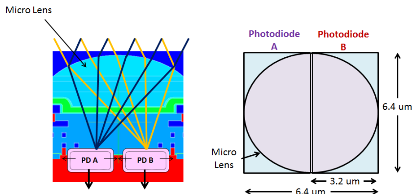
Figure 5 Showing the dual photodiode and microlens structure within a single photosite in the 4K CMOS image sensor used in the Cinema EOS cameras
