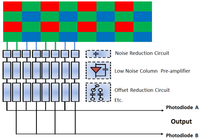
Figure 6 Showing the principle of the dual output from each individual photosite and the unique column readout circuits employed within the image sensor itself
