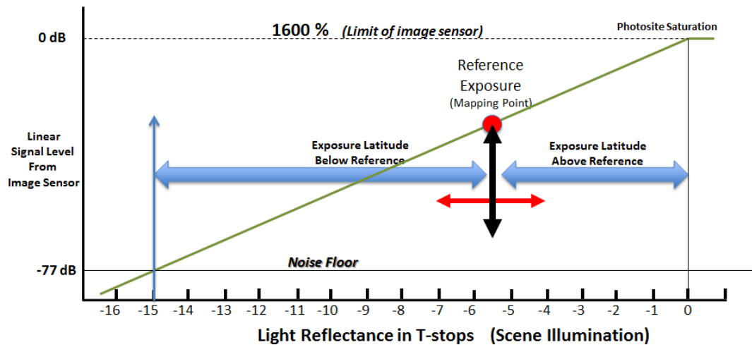
Figure 12 Illustrating the concept of the search for a mapping point for the camera deploying the CMOS image sensor shown in Figure 7
