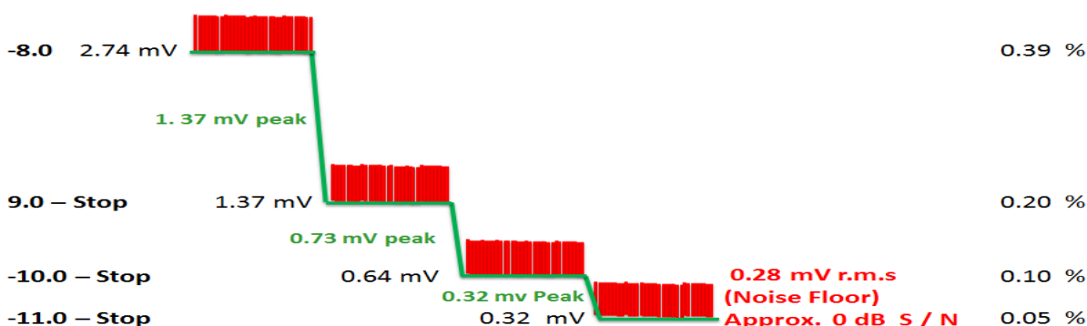
Figure 16 Illustrating the lower video signal levels (in millivolts) and the rms noise associated with the camera Luma specification of 68 dB that define the lower boundary to effective camera dynamic range
