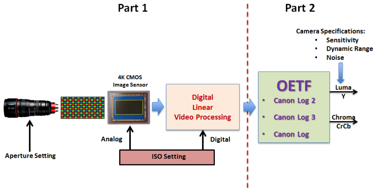
Figure 3 Showing the components either side of the image sensor that significantly influence how its dynamic range characteristic is mapped to produce the final camera specifications
