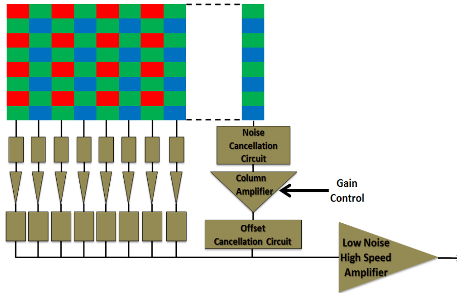
Figure 8 Highlighting the column structure for reading out the signal from the CMOS image sensor
