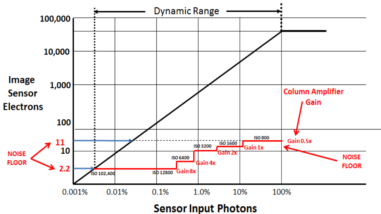
Figure 10 Increasing the amplification of the column amplifier progressively lowers the overall noise floor of the image sensor
