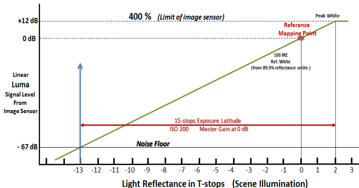
Figure 15 Showing the mapping that was decided upon for the EOS C700 and EOS C300 Mark II cameras on the linear light representation when set to originate HDTV video according to the ITU-R BT.709 production standard
