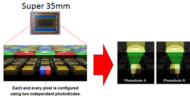
Figure 4 A representation of the dual pixel CMOS image sensor with a specially designed microlens that optimizes the focusing of the incident light onto both photodiodes
