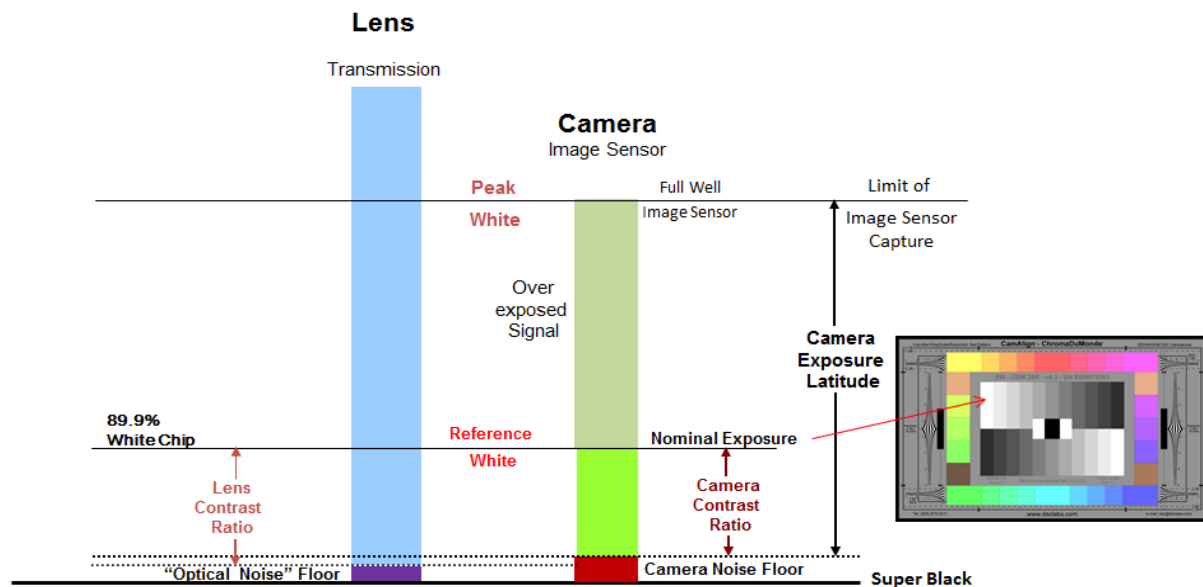
Figure 14 Traditional video exposure practices where the 89.9% reflectance chip on the gray scale chart is set by the lens aperture to produce 100 IRE level of Luma on a video waveform monitor
