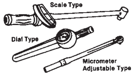
Figure 1-19 Torque Instruments
