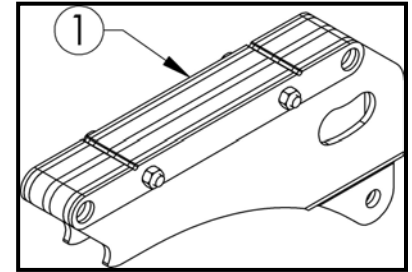
Assembled Detail
