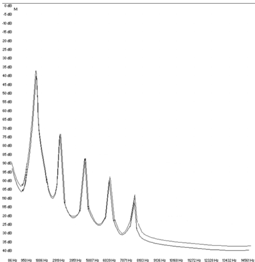
Comparison of Harmonics generated by the filter circuits of the Prophet-V2.5 and Prophet 5 when in self oscillation
