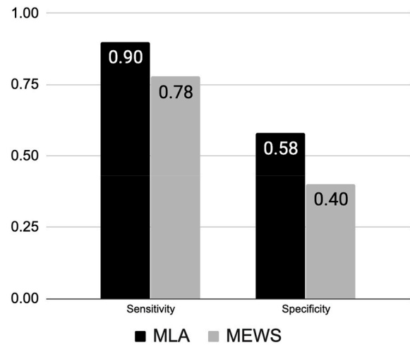
Fig. 2. Comparison of sensitivity and specificity for the machine learning algorithm and MEWS score. Abbreviations: MLA: Machine Learning Algorithm. MEWS: Modified Early Warning Score.
