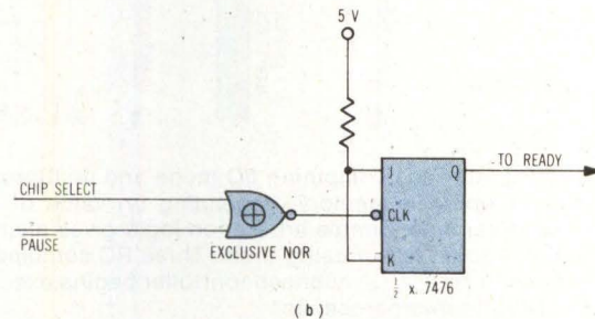
Fig 3 Timing diagram. In (a), both APU and NCU must generate ready input to microprocessor shortly after address strobe is issued. For NCU, digit address strobe (DAS) clears ready so processor can complete its cycle. If APU uses extended read/write strobes, PAUSE can serve as ready input; otherwise, in (b), Q output of J-K flipflop in toggling mode goes low at chip select falling edge and high on rising edge of PAUSE
