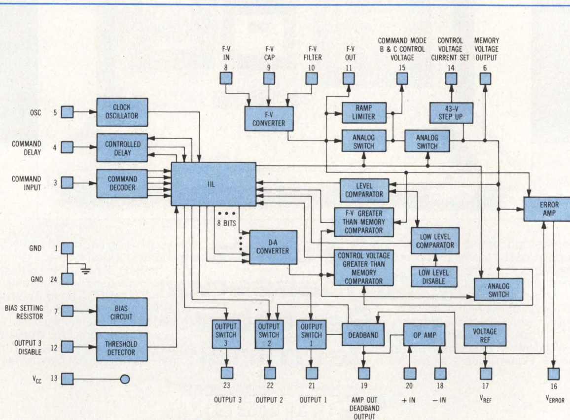
Universal analog controller, NE5522N, from Signetics is implemented in LSI. Chip is used for industrial applications involving closed loop control of machine speed and acceleration
