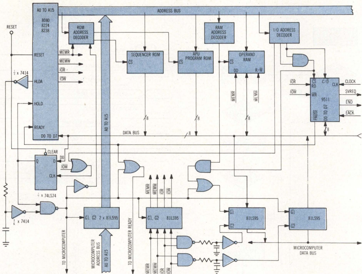
Fig 4 APU interface combining I/O mode and multiprocessor mode. Either APU sequencer/controller or microcomputer can access operand memory, depending on value of HLDA. Five buffers isolate buses on APU side from buses on microcomputer side. Simple arbitration logic gives microcomputer access to buses on APU side if HLDA shows that sequencer/controller is not using them. Three RC combinations add synchronization delay. RESET clears hold flipflop, and HLDA goes to zero, as sequencer/controller begins execution. Halt instruction writes APU status to RAM and returns control of buses to microprocessor
