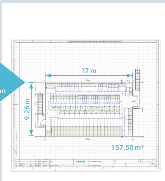
Optimized layout
