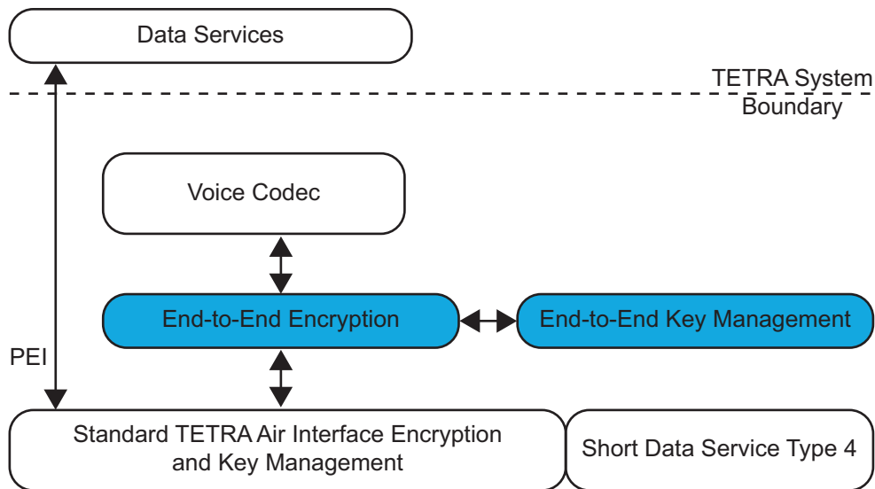
Figure 7: Voice and Data End to End Encryption
