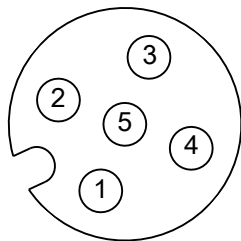
Fig. 12: M12 socket
