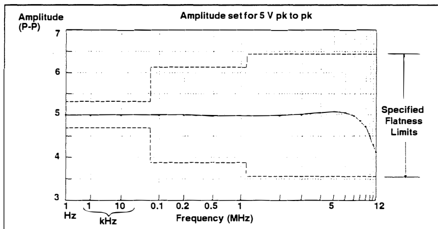
Fig. 1-3. Typical Amplitude Flatness for Sine Wave
