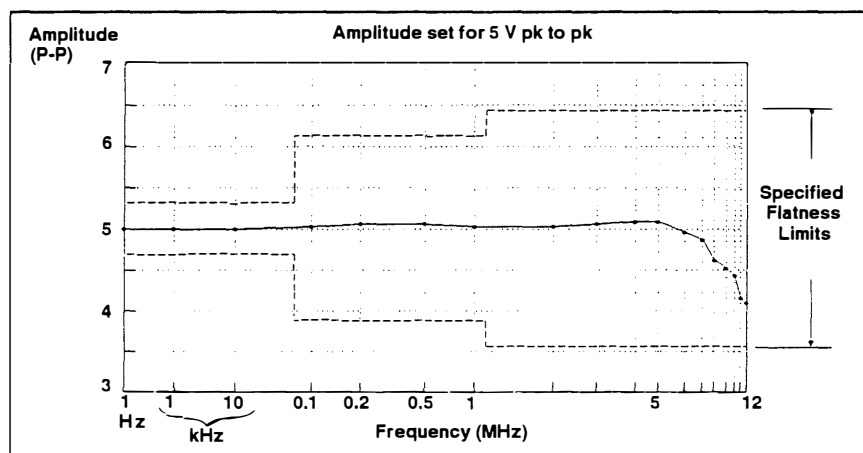
Fig. 1-5. Typical Amplitude Flatness for Triangle Wave
