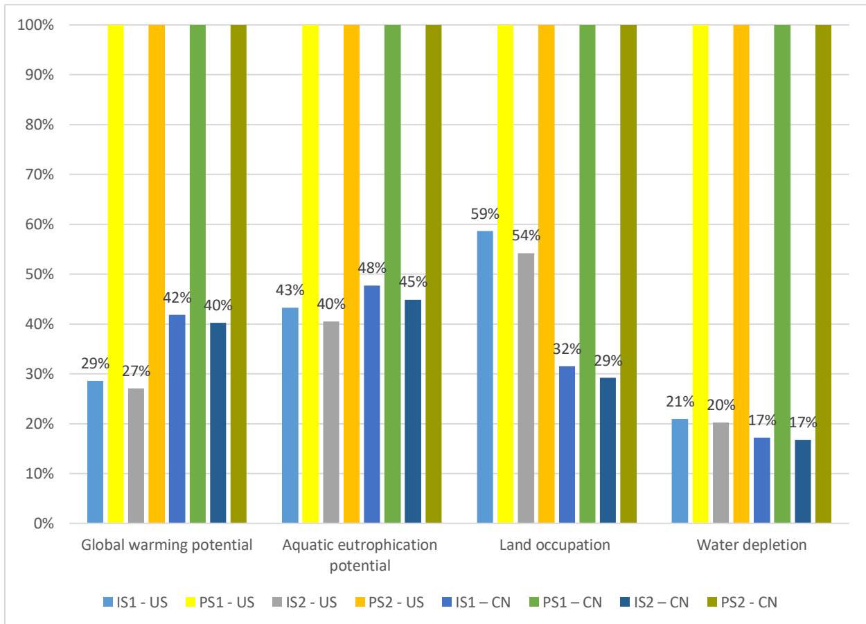
Figure 1 - Environmental indicators of the IS scenarios against the PS patty scenarios. Note the maximum of the two pairs (i.e., IS1 - US and PS1 - US; IS2 - US and PS2 - US) is indicated at 100%.
