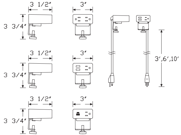
Surface Clamp
