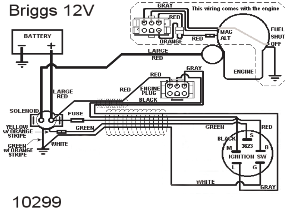
WIRING DIAGRAM ( QBRT14544 ) FIGURE 11
