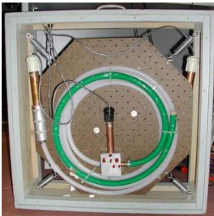
Figure 92. The opened acoustic module and the complete system
