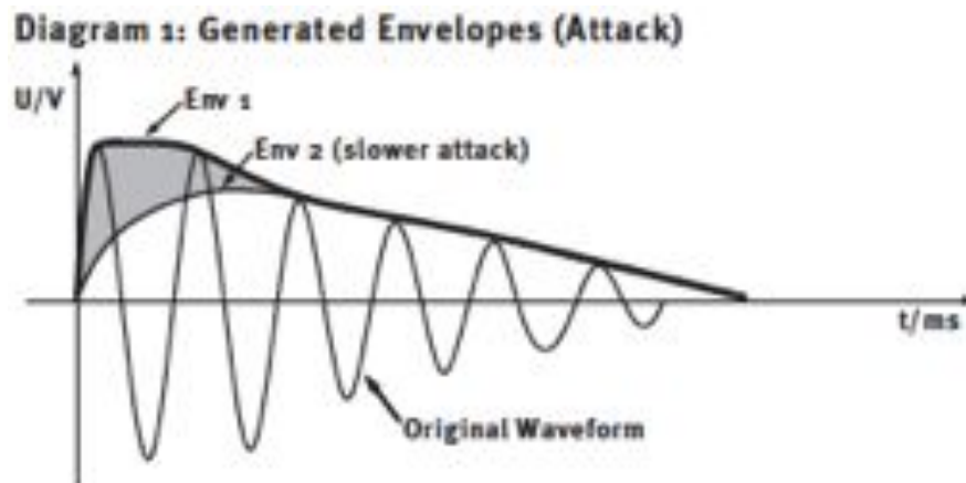
Figure 119. SPL Transient Designer Attack Envelopes
