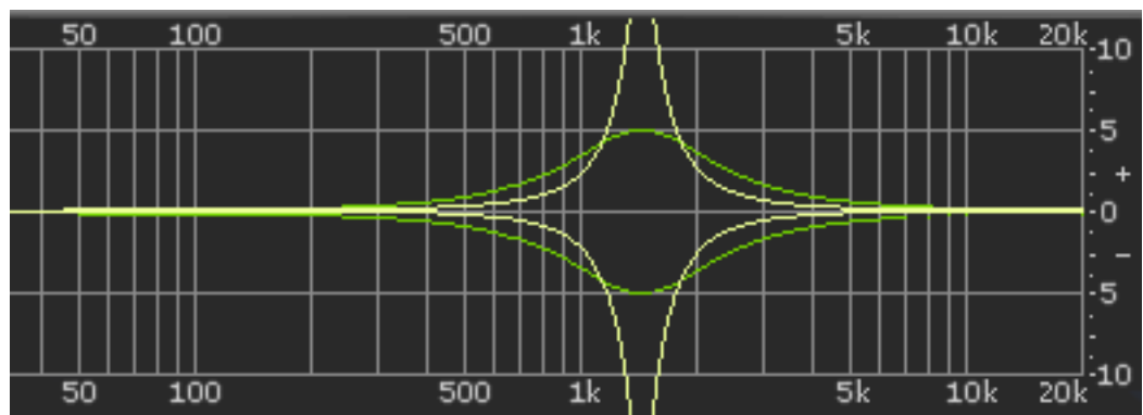
Figure 65. Parametric Type III response
