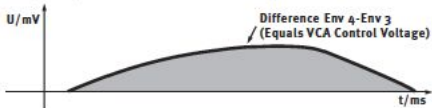
Figure 123. SPL Transient Designer Sustain Control Voltage
