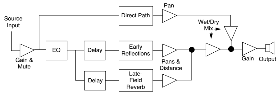
Figure 93. RealVerb Pro signal flow
