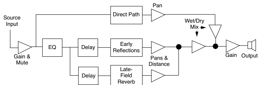
Figure 104. DreamVerb signal flow
