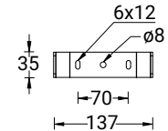
Mounting detail
