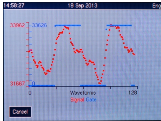
Marginal Waveform
