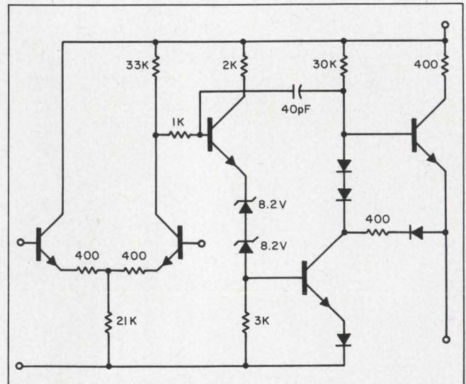
The capacitor and diodes for the summing amplifier are formed from a parallel resistor combination and transistor base-emitter junctions.
