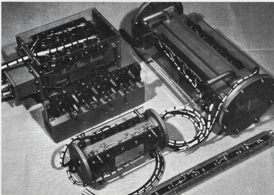
Ferrite phase-shifters on display . . . 34
