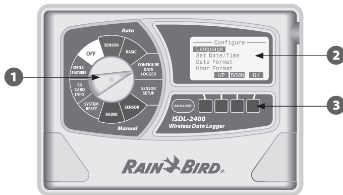
Figure 3 - ISDL-2400 Wireless Data Logger
