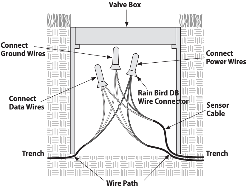
Figure 11 - Valve Box Wiring Diagram
