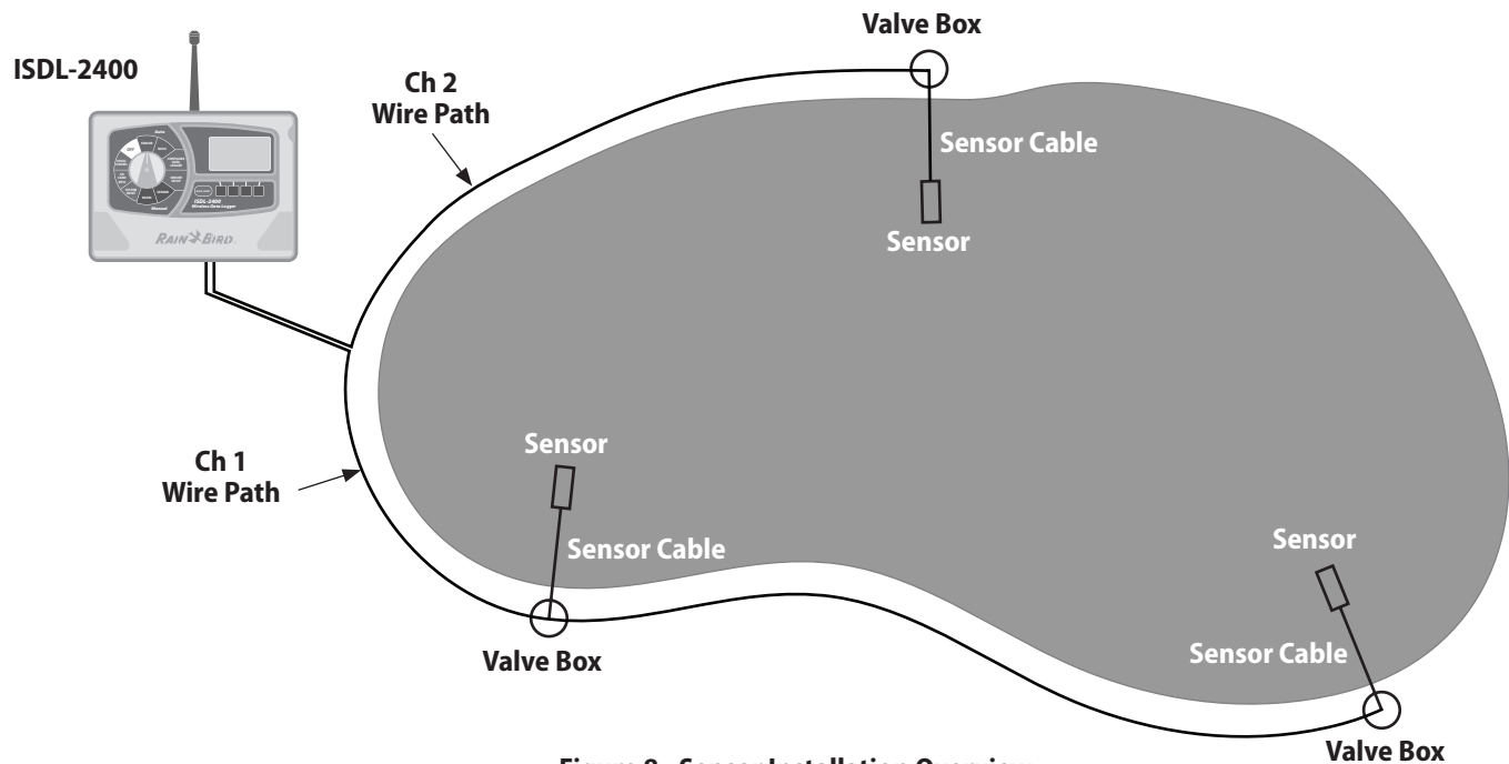
Figure 8 - Sensor Installation Overview
