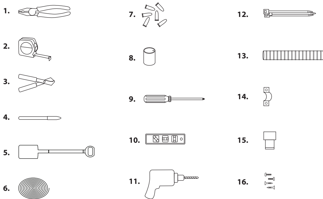
Figure 7 - Installation Tools
