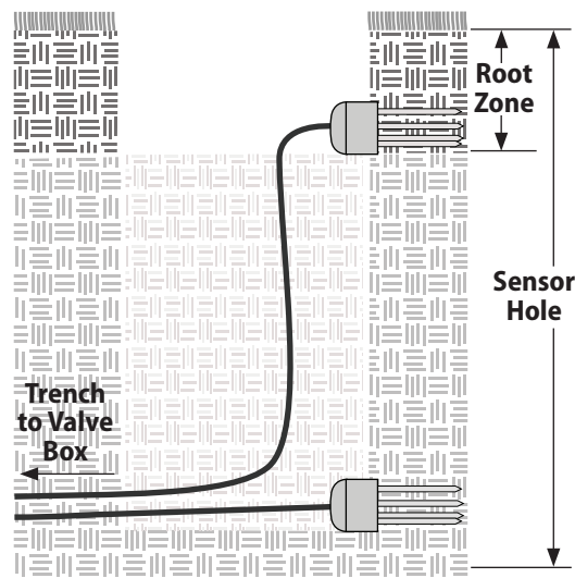
Figure 9 - Type 3 Sensor Installation
