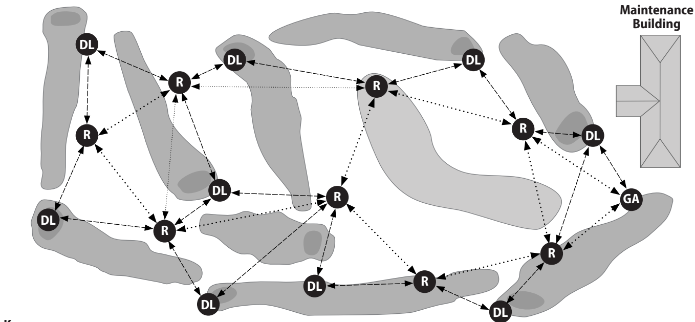
Figure 6 - Site Survey Location Example
