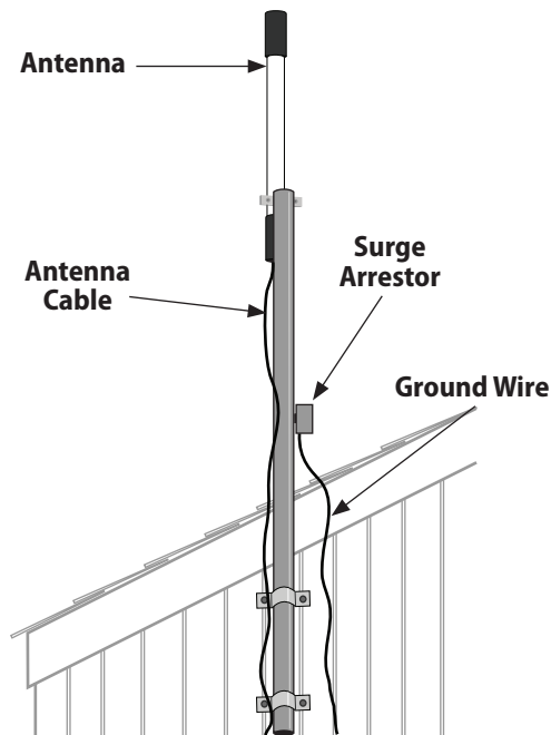
Figure 13 - Antenna Installation
