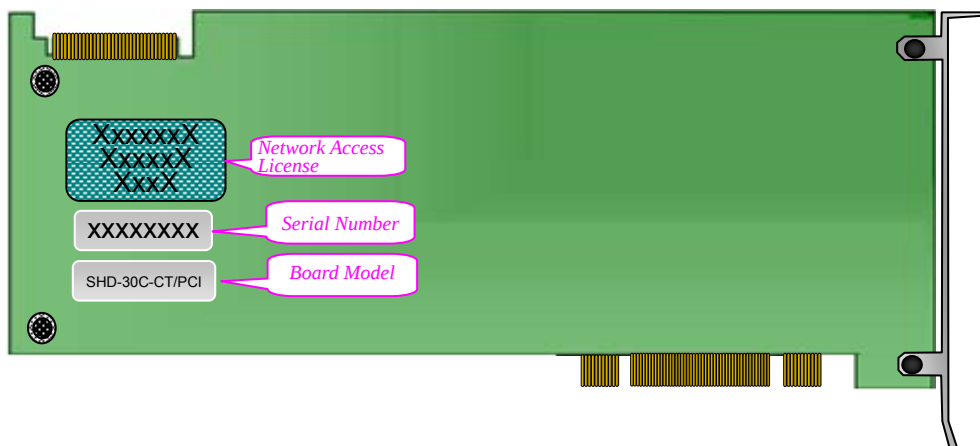
Figure 2-2 Rear View
