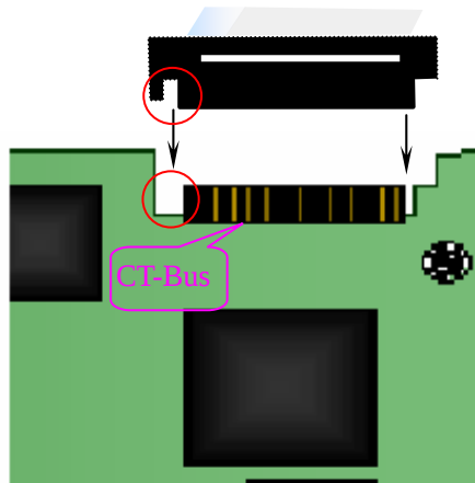
Figure 2-11 Connection of H.100 Bus
