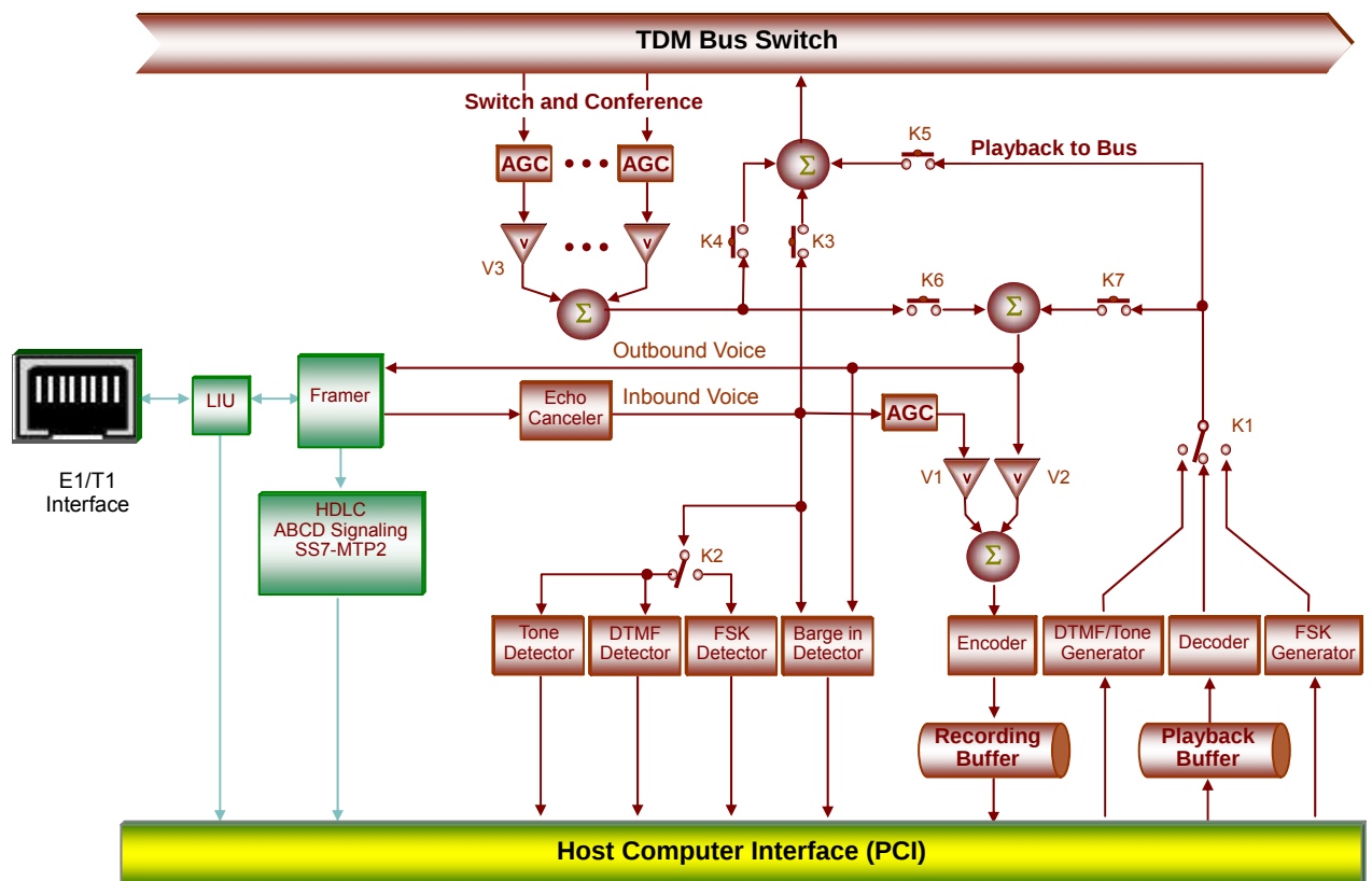
Figure 1-1 Operation Principle
