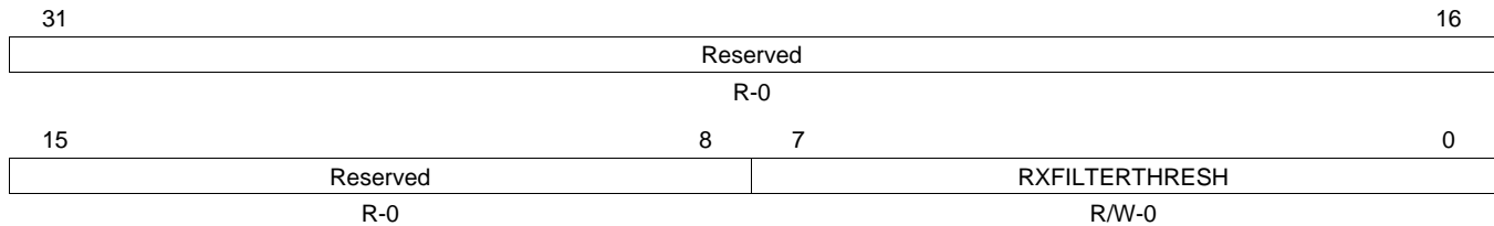
Figure 54. Receive Filter Low Priority Frame Threshold Register (RXFILTERLOWTHRESH)
