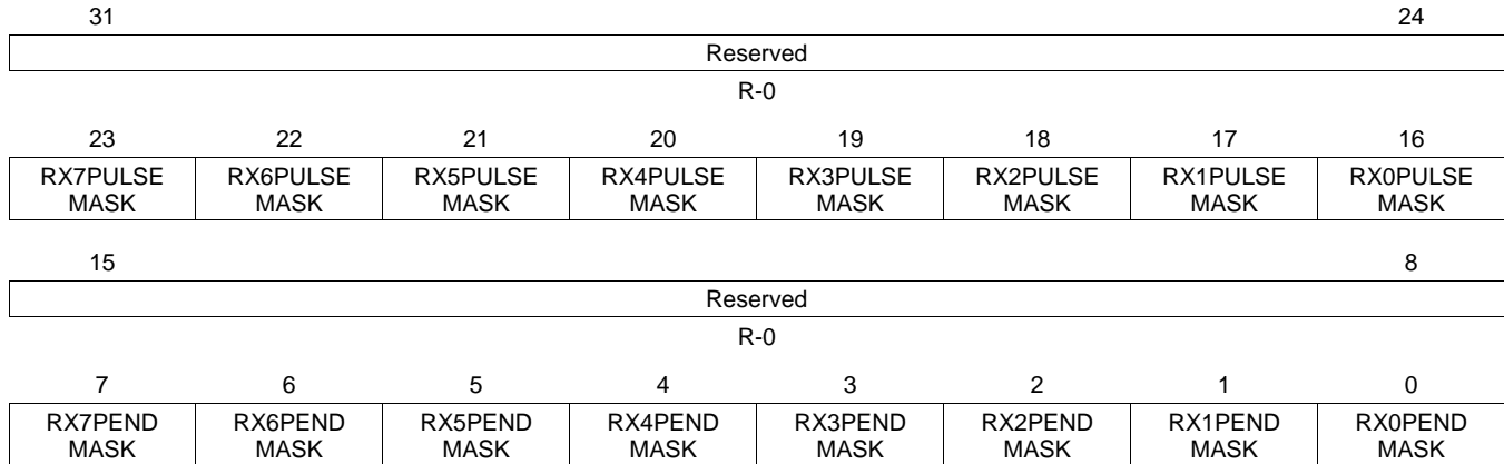
Figure 43. Receive Interrupt Mask Set Register (RXINTMASKSET)
