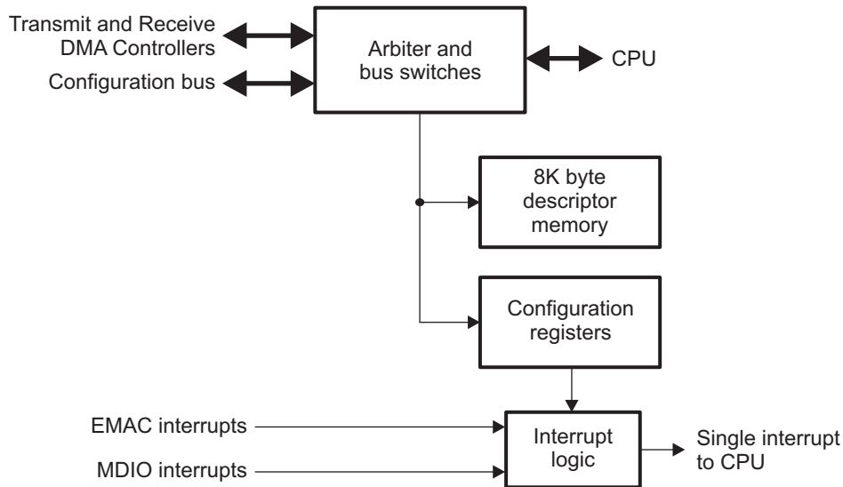
Figure 11. EMAC Control Module Block Diagram
