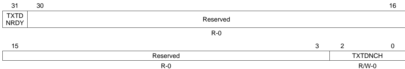
Figure 32. Transmit Teardown Register (TXTEARDOWN)
