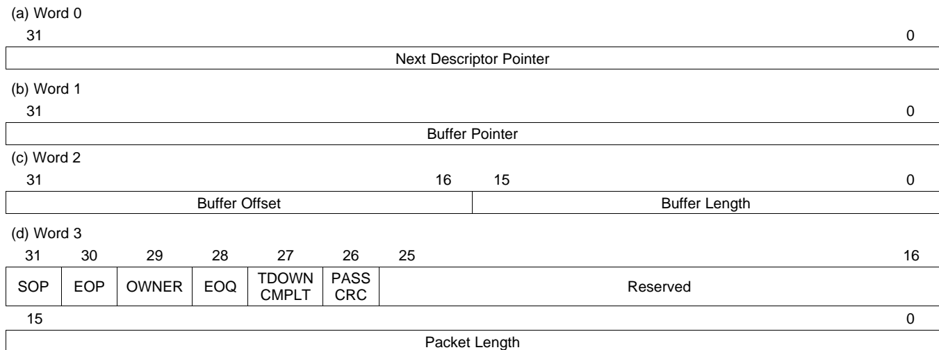
Figure 9. Transmit Descriptor Format
