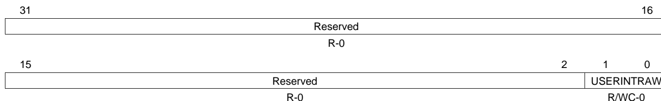
Figure 22. MDIO User Command Complete Interrupt (Unmasked) Register (USERINTRAW)
