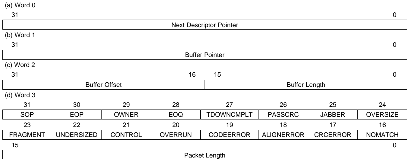
Figure 10. Receive Descriptor Format
