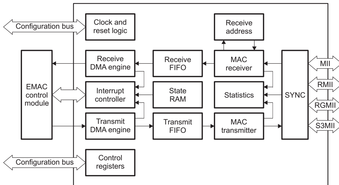
Figure 13. EMAC Module Block Diagram
