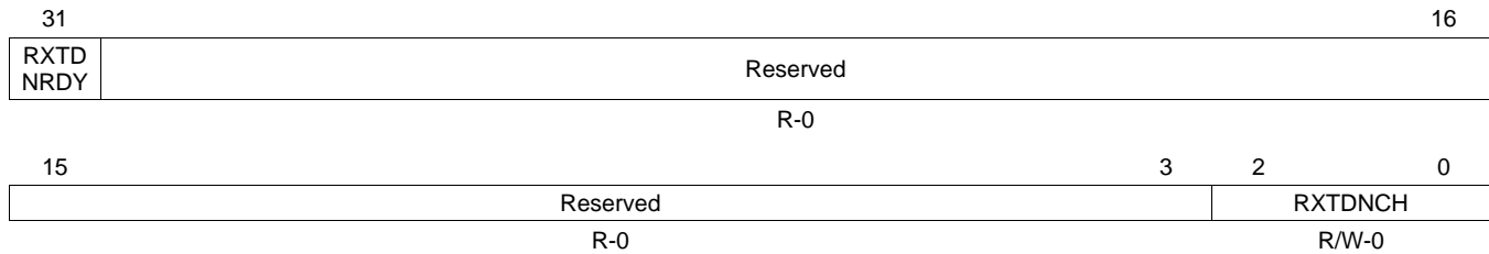
Figure 35. Receive Teardown Register (RXTEARDOWN)
