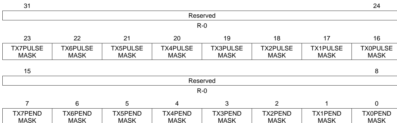
Figure 38. Transmit Interrupt Mask Set Register (TXINTMASKSET)
