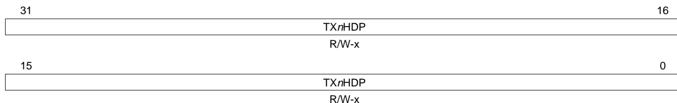
Figure 74. Transmit Channel n DMA Head Descriptor Pointer Register (TXnHDP)
