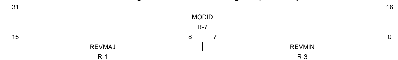
Figure 16. MDIO Version Register (VERSION)
