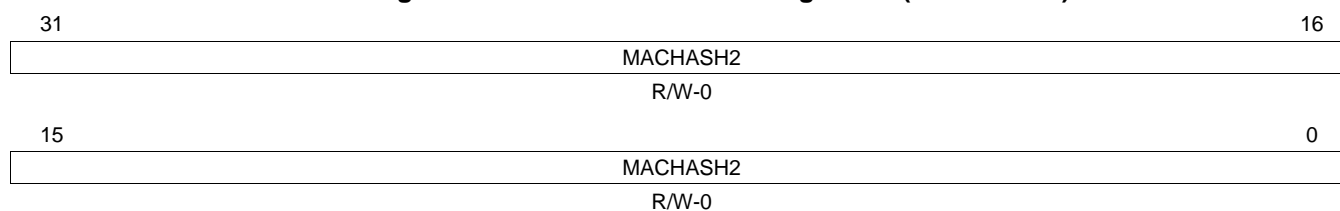
Figure 66. MAC Hash Address Register 2 (MACHASH2)
