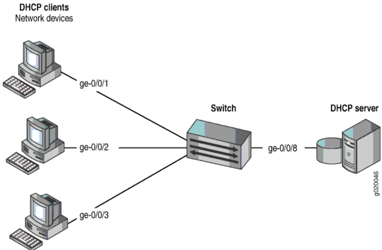
Figure 1: Network Topology for Basic Port Security
