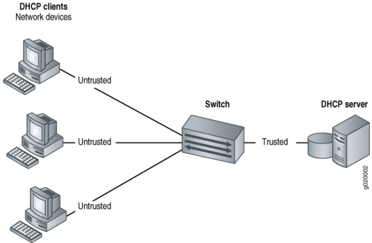
Figure 18: DHCP Server Connected Directly to a Switch
