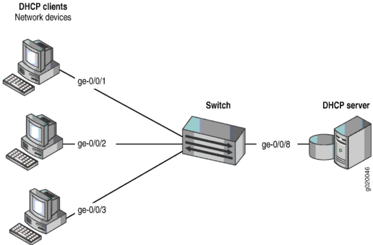
Figure 33: Network Topology for Basic Port Security
