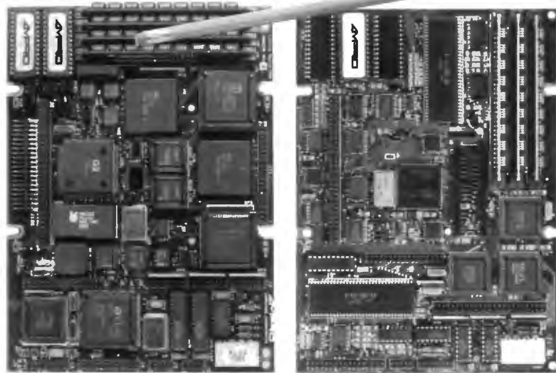
Little Board™/286
