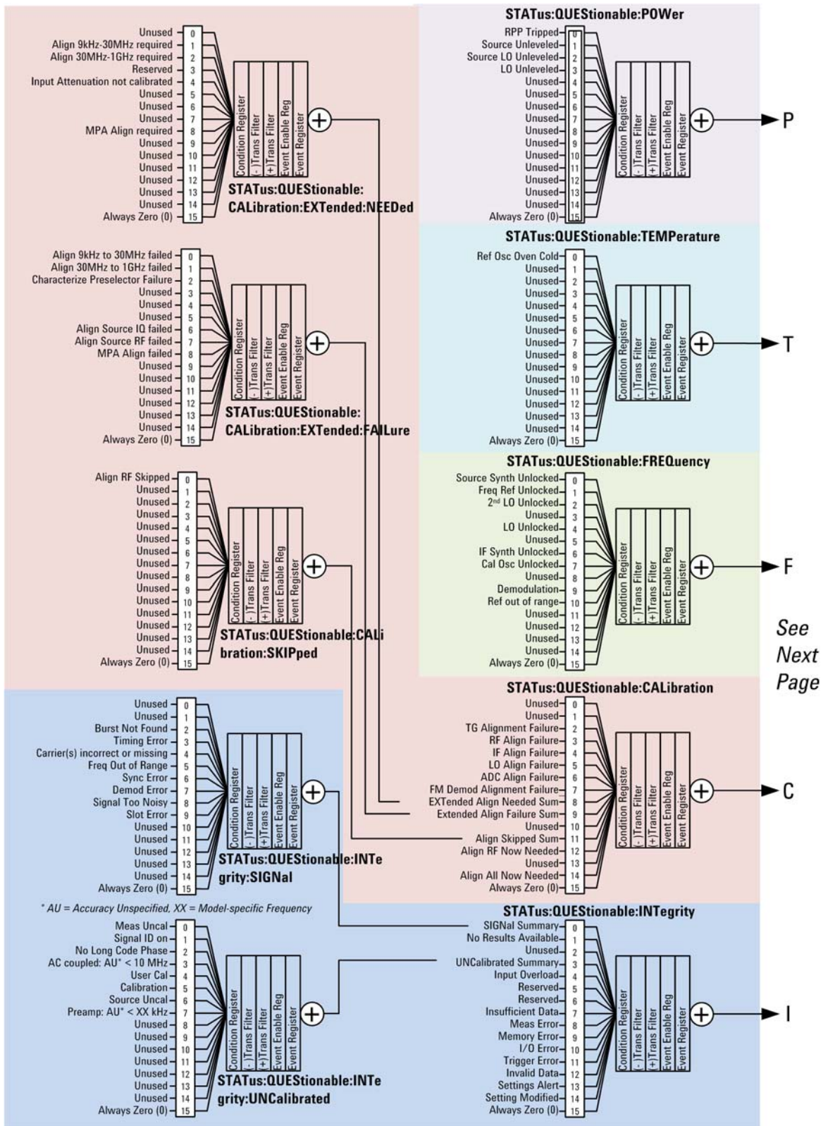
X-Series Status Register System
