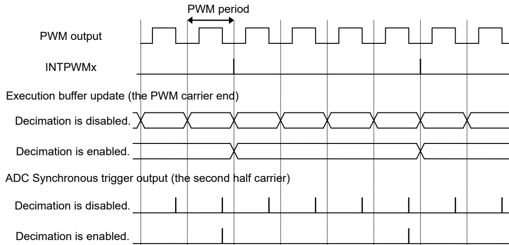
Figure 3.18 Timing example of Decimation control (in the case of \langle \text{INTPRD}[1:0] \rangle = 11 )
