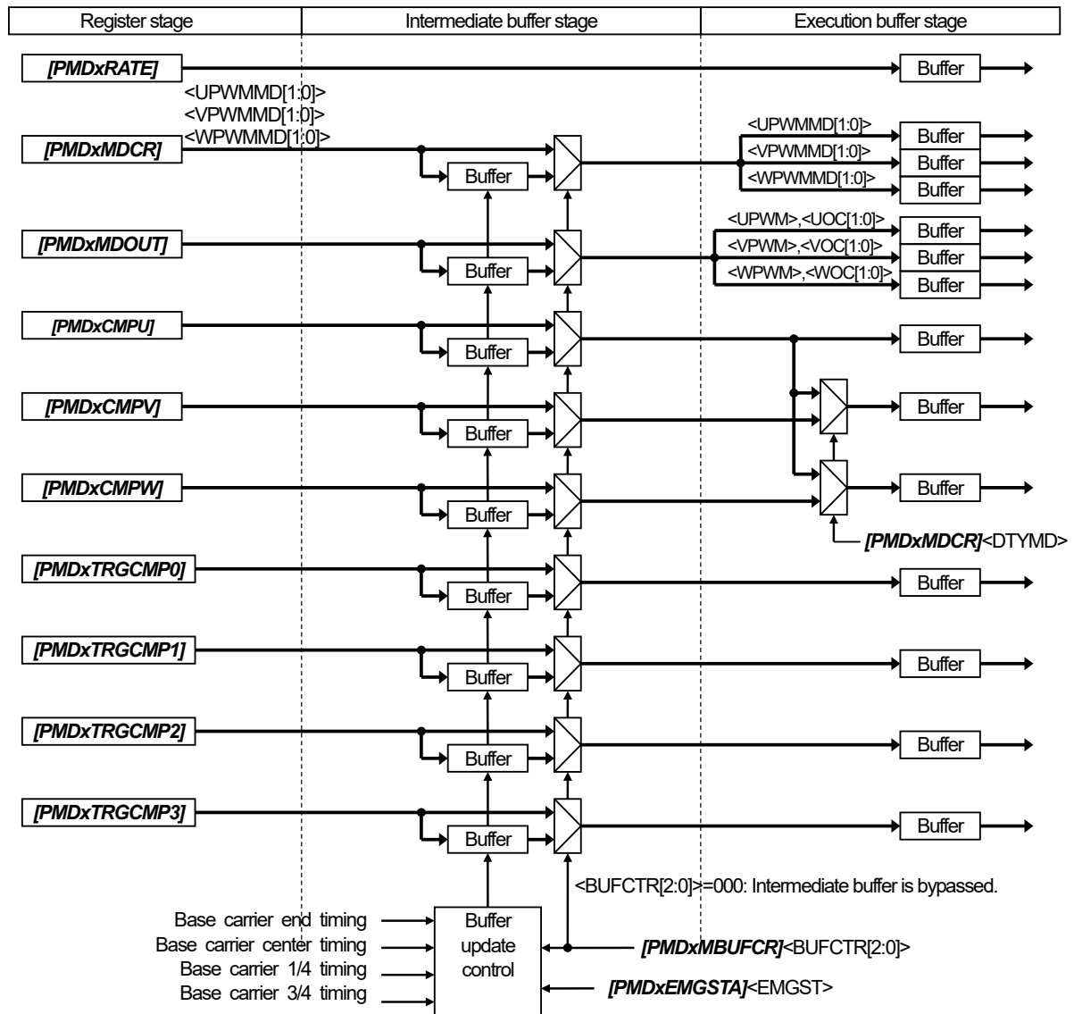
Figure 3.17 Register buffer configuration
