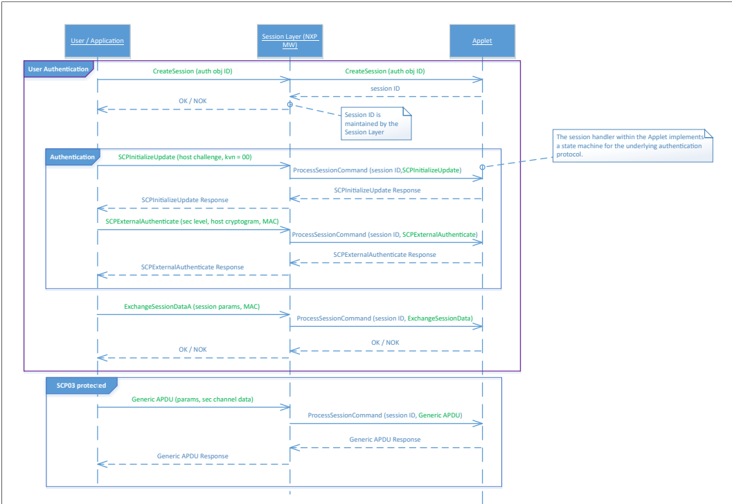
Figure 10. Session creation using an AES key as authentication object
