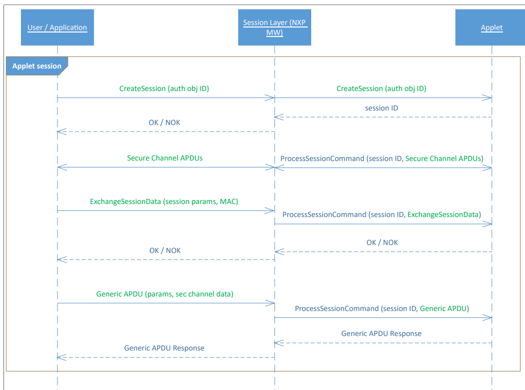
Figure 8. Applet session (overview)
