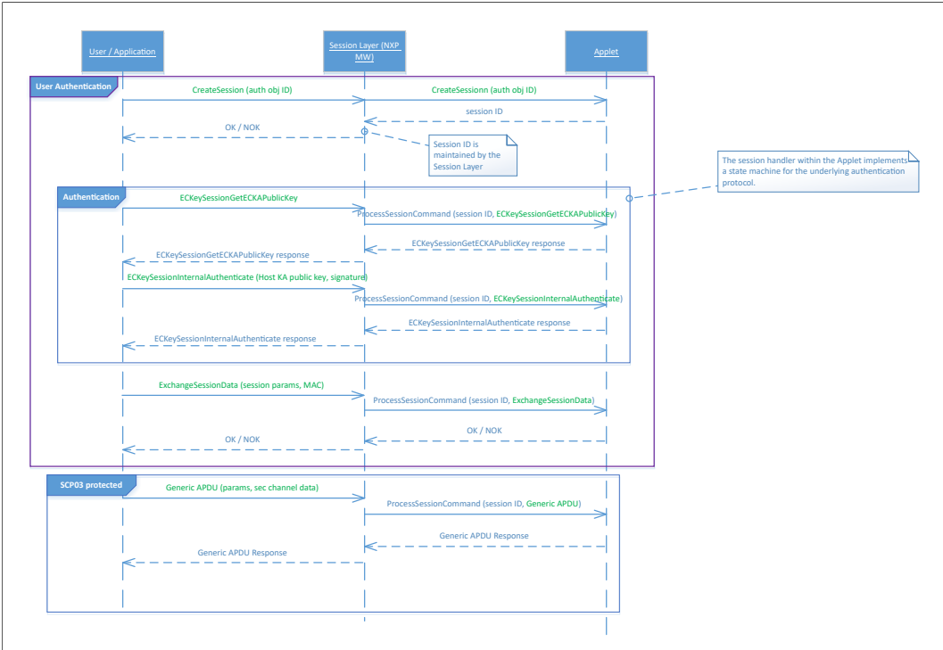
Figure 11. Session creation using ECKey session as authentication mechanism.
