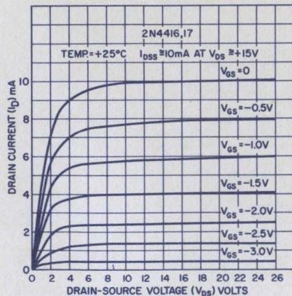
DRAIN CURRENT VS. DRAIN-SOURCE VOLTAGE
