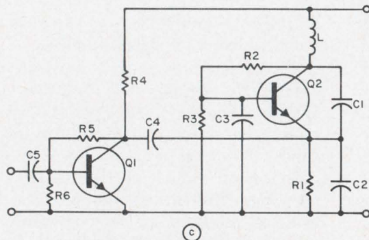
Bandwidths of several kHz are possible with these two configurations. One is a common-base Colpitts (c) and the other a common-base Hartley (d). Both use the voltage-sensitive capacitance between the emitter and base of transistor Q2 to frequency-modulate the carrier. These circuits are used to transmit signals such as electrocardiograms and electromyograms from a few feet up to about 100 feet.
