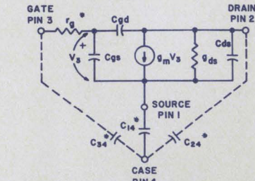
Approximate small signal equivalent circuit for the 2N4416 Field Effect Transistor.
