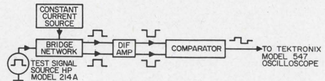
1. Diode capacitance and dynamic resistance test set can be built quickly, as this block diagram shows.
