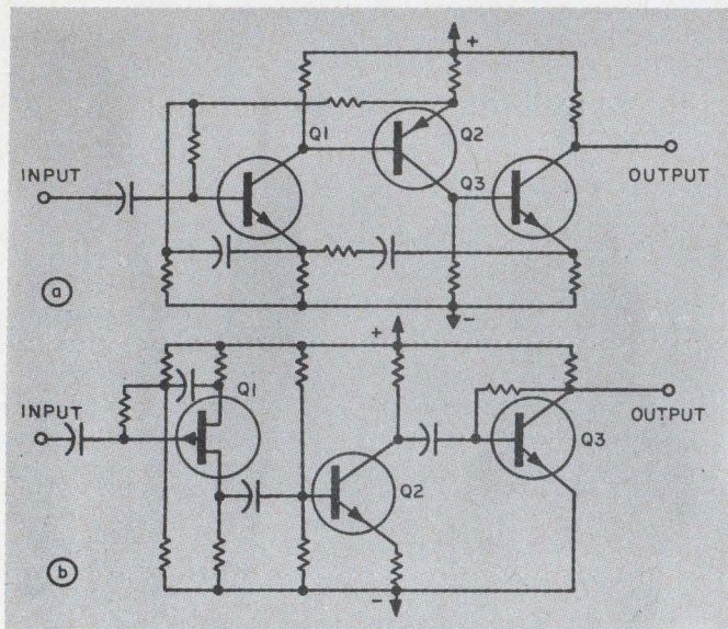
4. Two techniques for obtaining high input impedance in amplifiers and preamplifiers are bootstrapping and the use of FET input stages. In (a), an input impedance of 1 MΩ is achieved by use of a bootstrapped bias network for transistor Q1. In (b), a 10-MΩ input impedance to the amplifier is obtained by using both bootstrapping and a FET input stage.
