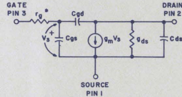
Approximate small signal equivalent circuit for the 2N4417 Field Effect Transistor.
