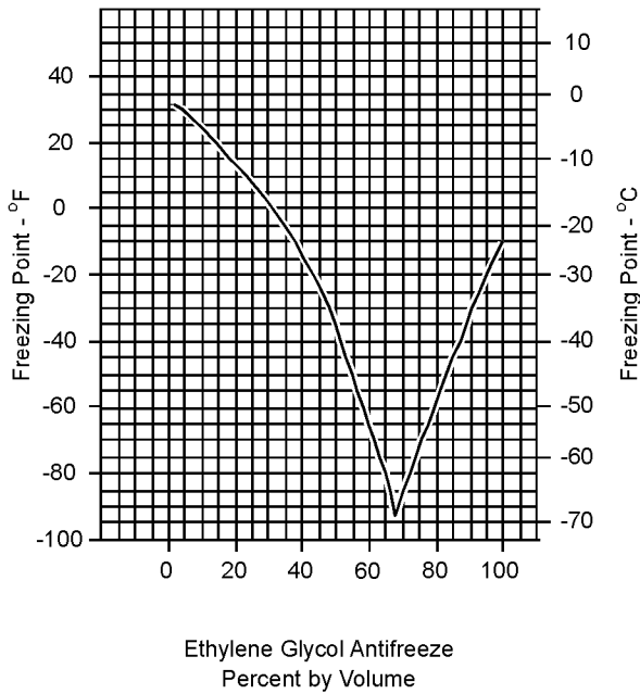
Illustration 3 g03387377 Approximate curve of the freezing point for a typical ethylene glycol solution.
