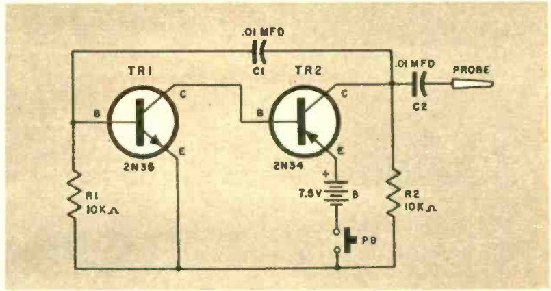
Two transistor amplifier using capacitive feedback to make multivibrator.
