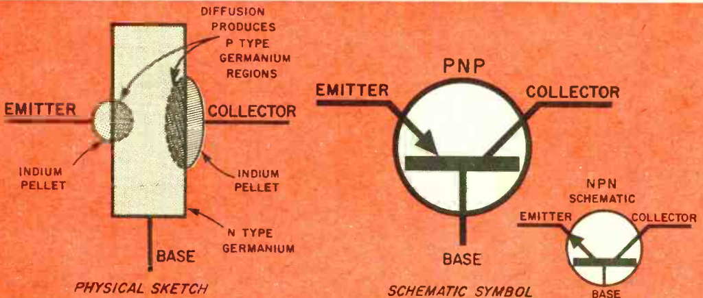
Fig. 1. At left is a physical representation of a transistor showing its basic semiconductor material composition. Standard symbols are at right.
