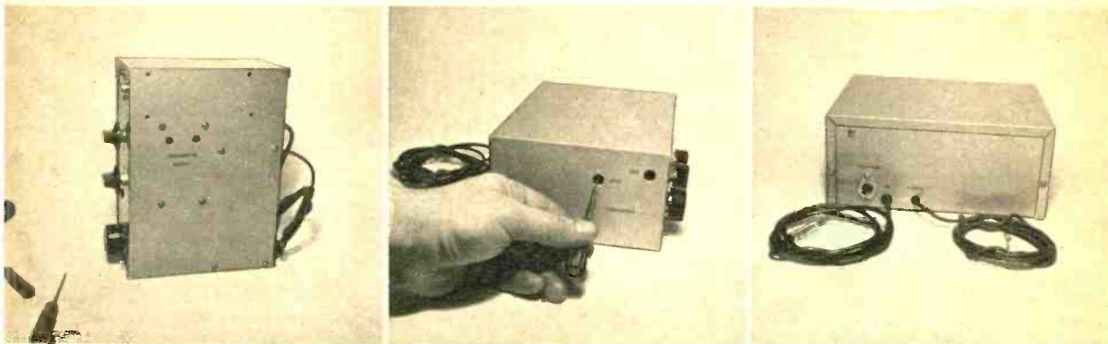
Bottom, side and rear views of completed unit shows position of holes to be drilled. Rear of unit contains auto antenna plug, and input and output cables.
