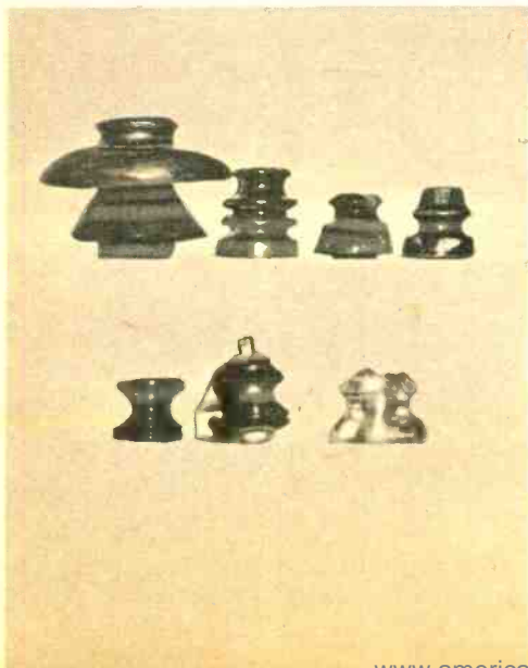
Top (l to r): 34,000-v two skirts; 16,000-v top groove; 7200-v top groove; 2300-v side groove. Bottom: 117-v spool used with secondary; same with support; glass telephone insulator.
