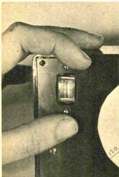
A miniature AM tuning meter provides accurate reading of wattage when properly calibrated. An inked-in scratch marks its "null" point. Simple coil serves as high-current, low-resistance input shunt resistor.
