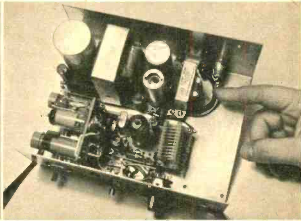
Power supply is shown mounted in chassis. All modules except modulator are also visible.
