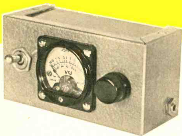
Many of the components shown in the wiring guide above are miniaturized to fit easily into the compact case. A separate subchassis is not needed.
