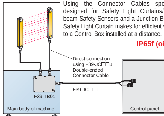
F39-TB01 Junction Box for Safety Light Curtain
