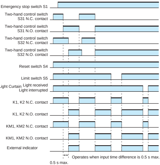
Timing Chart
