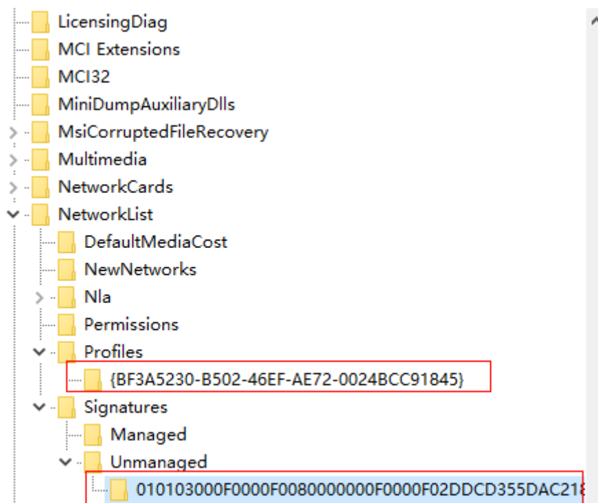
Figure 6-1 Registry directory
