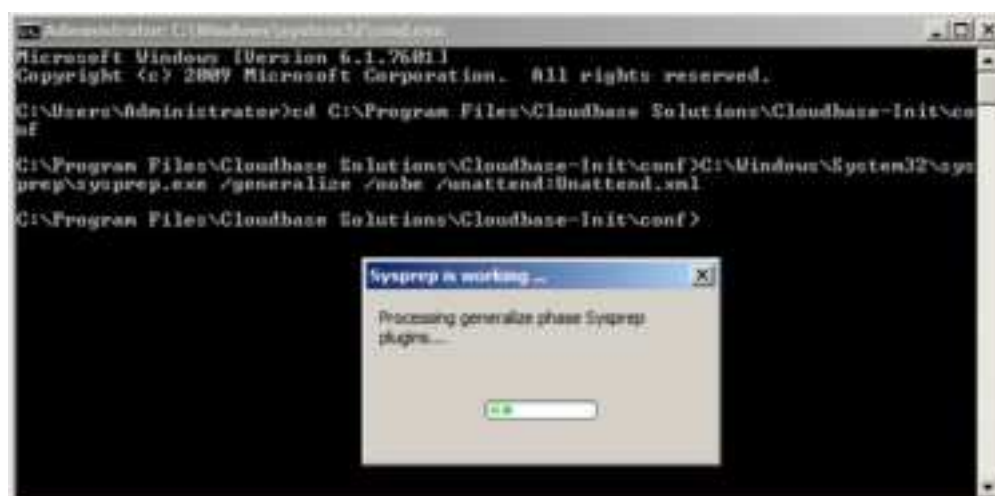
Figure 4-8 Running Sysprep
