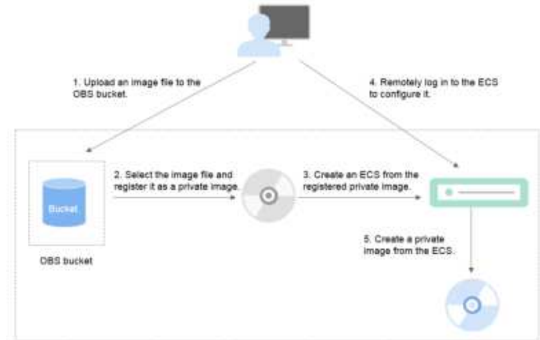
Figure 6-4 Image creation process
