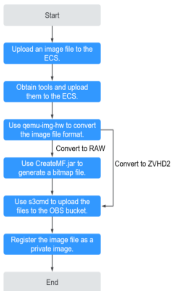
Figure 2-5 Import process (Linux)
