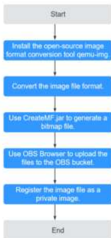
Figure 2-6 Import process (Windows)
