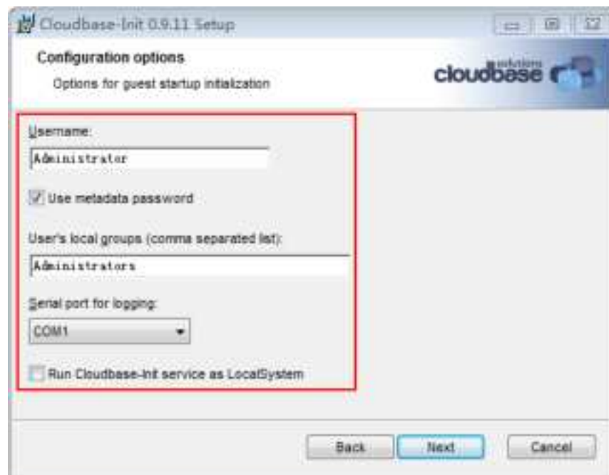
Figure 4-5 Configuring parameters
