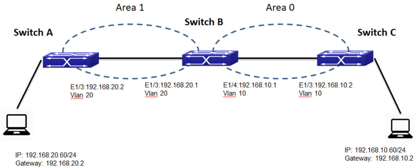
Figure 4-9-4-13 Network topology of OSPF autonomous system
