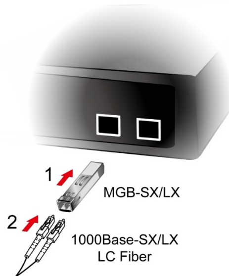
Figure 2-2-4: Plug-in the SFP/SFP+ Transceiver
