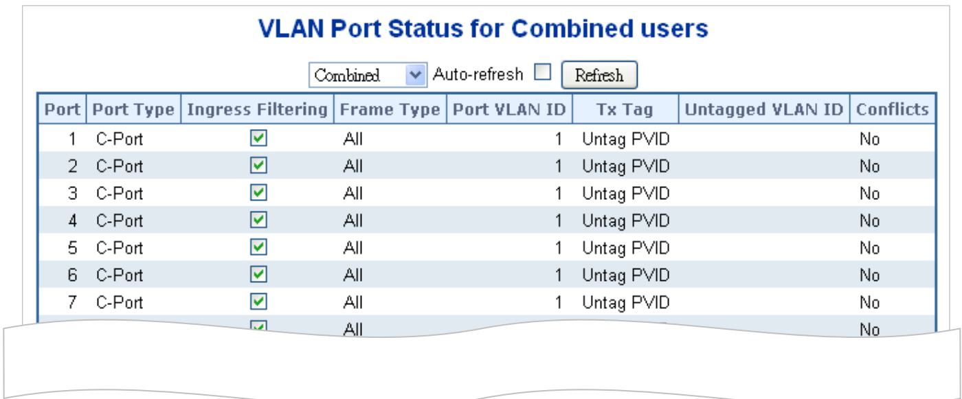
Figure 4-3-3-4: VLAN Port Status for Combined users Page Screenshot
