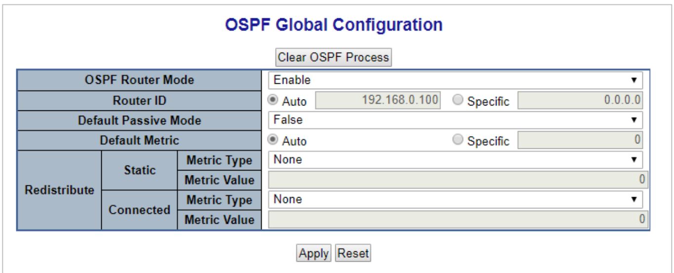
Figure 4-9-4-1: OSPF Global Configuration Page Screenshot
