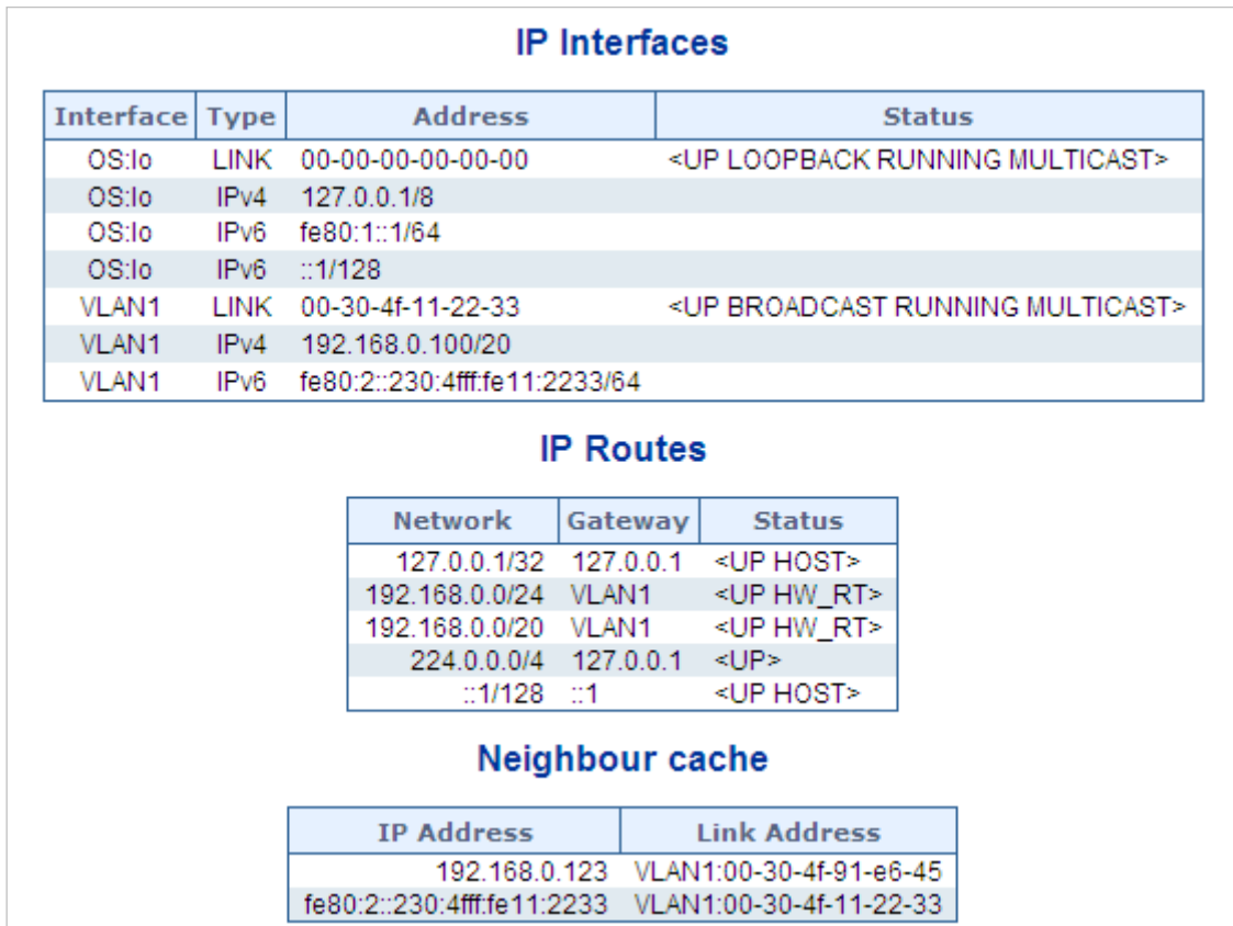
Figure 4-9-2: IP Status Page Screenshot
