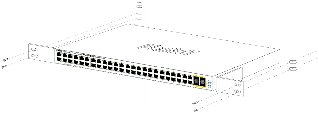
Figure 2-2-3: Mounting Managed Switch in a Rack
