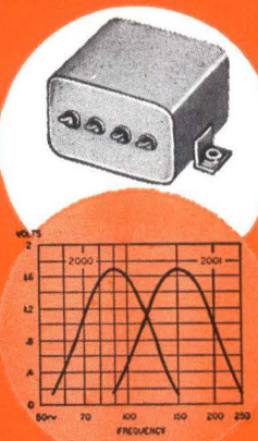
Curves of our miniaturized 90 and 150 cycle filters for glide path systems. 1\frac{1}{4}'' x 1\frac{1}{4}'' x 1\frac{1}{8}'' .
