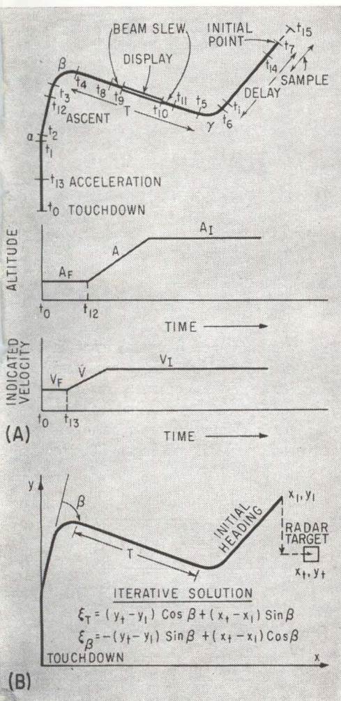
TYPICAL FLIGHT course (A) generated by system iterates its simulations until it generates final course—Fig. 7
