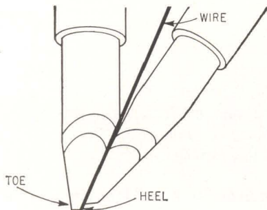
GROOVE in bonding surface of bonding tool's left jewel goes from toe to heel and up side. Wire-feed tube is formed when other jewel is clamped against first—Fig. 1
