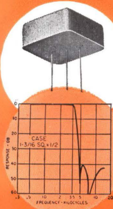
Miniaturized 3.5 KC low pass filter. 10K ohms to 10K ohms. Within 1 db up to 3500 cycles. Greater than 40 db beyond 4800 cycles.
