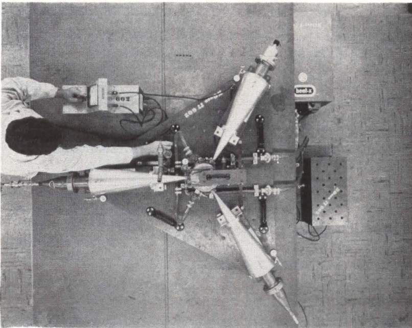
HIGHEST level of operation attained by Y-circulator is claimed for experimental model shown above. Model was designed for shipboard radar, enables transmission and reception on same antenna. Unit was designed and built by Electronic Communications, Inc., further work is now in progress on other versions
