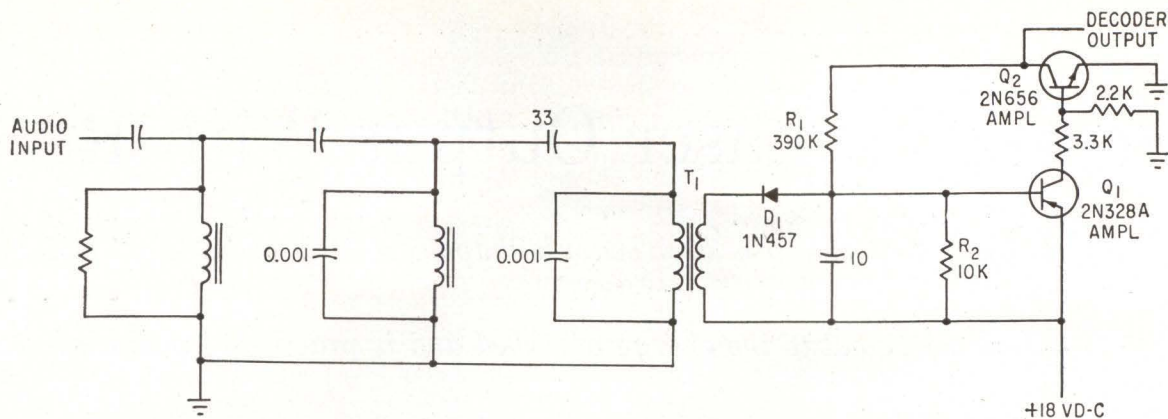
THERE ARE 20 similar decoders in the system, each tuned to its particular frequency and operating its own relay—Fig. 4
