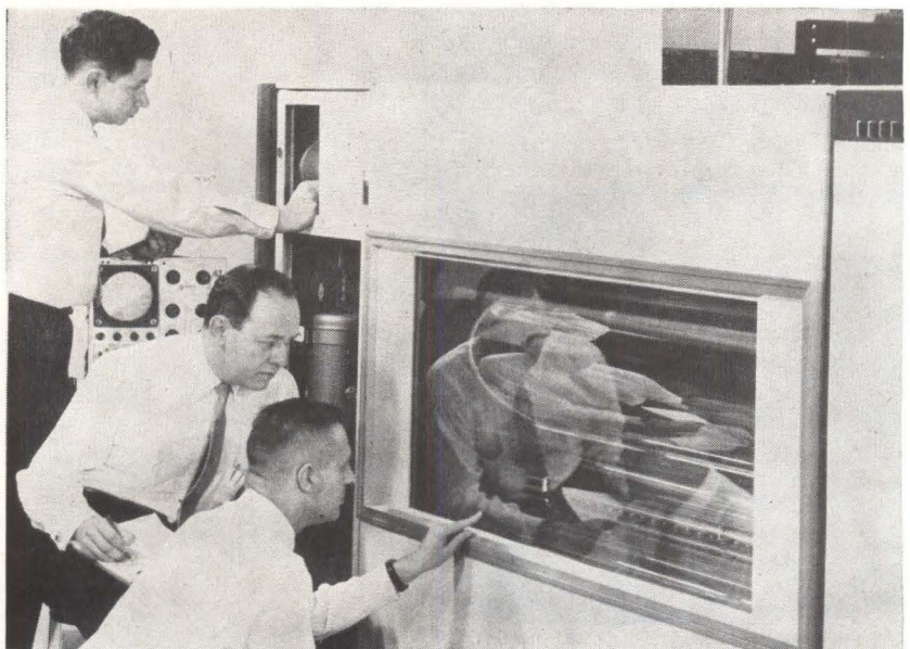
MASS STORAGE system announced by Univac can store 64.9 million characters of information and deliver them in 92 \mu sec. It has two drums rotating at 870 rpm and searched by 54 flying heads. Theoretically, 96 of these units can be used with a Univac 490 computer
