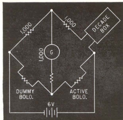
BRIDGE CIRCUIT of rat's nest calorimeter—Fig. 1
