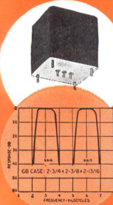
Three KC and 6 KC flat top band pass filters. 400 ohms to 20K ohms. MIL-T-27A; each filter 1.7 lbs.
