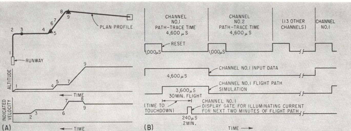
FLIGHT PATH profiles are shown in (A) for plane flying in the terminal area. Commutated data from different flight paths (B) goes to computer—Fig. 4
