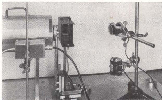
CALORIMETER SETUP: to calibrate scattering wire and phototube (left); to calibrate a second calorimeter, using an integral beam-splitter (right)—Fig. 2
