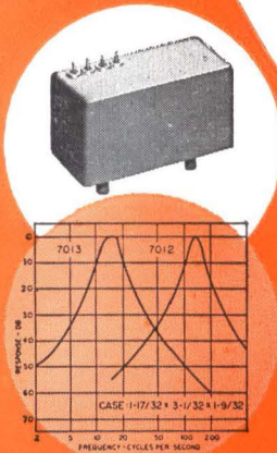
Fifteen cycle and 135 cycle filters for Tacan. 600 ohms to high impedance. Extreme stability -55^{\circ}\text{C.} to +100^{\circ}\text{C.}
