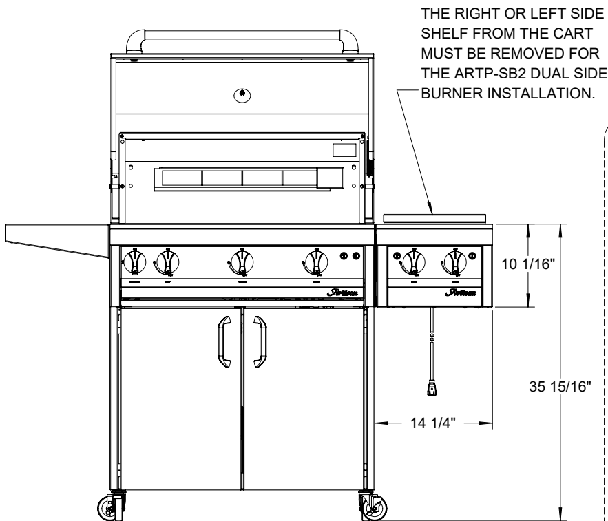
ARTP CART INSTALLATION DIMENSIONS
