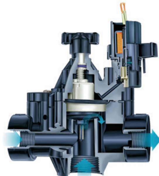
PGA Cutaway
