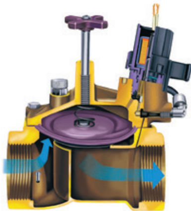
EFB-CP Cutaway
