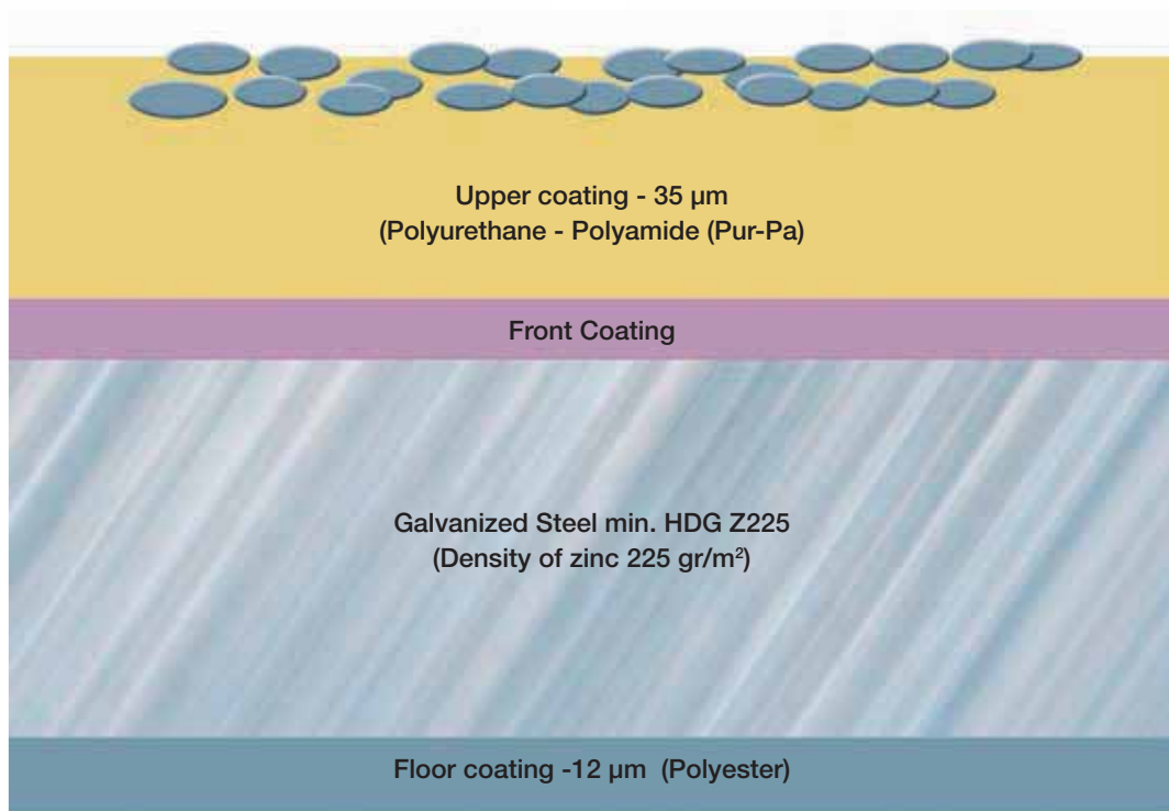
Panel coating
