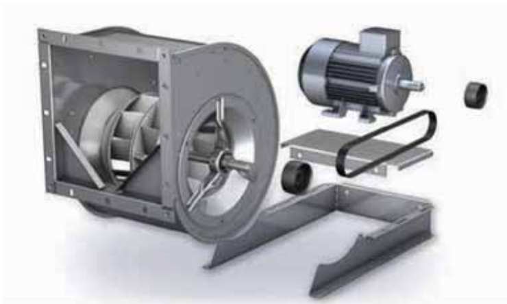
Belt-driven fans
