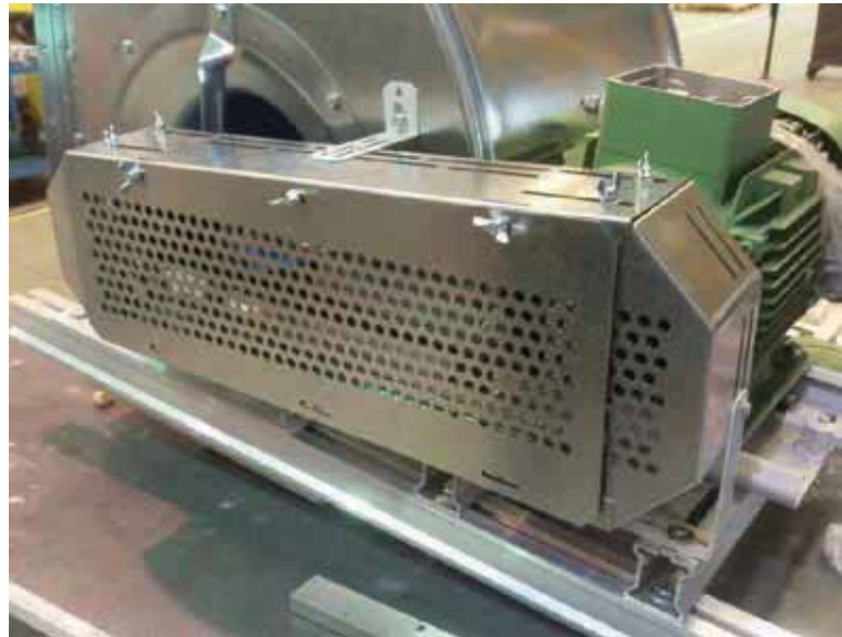
Drive guard (closed)
