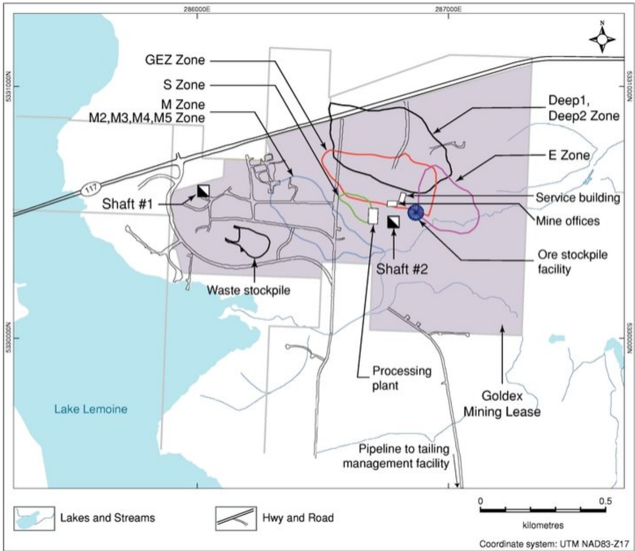
Surface Plan of the Goldex Mine (as at December 31, 2017)
