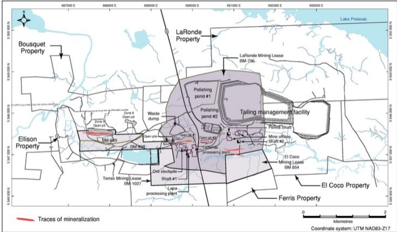
Surface Plan of the LaRonde Mine (as at December 31, 2017)
