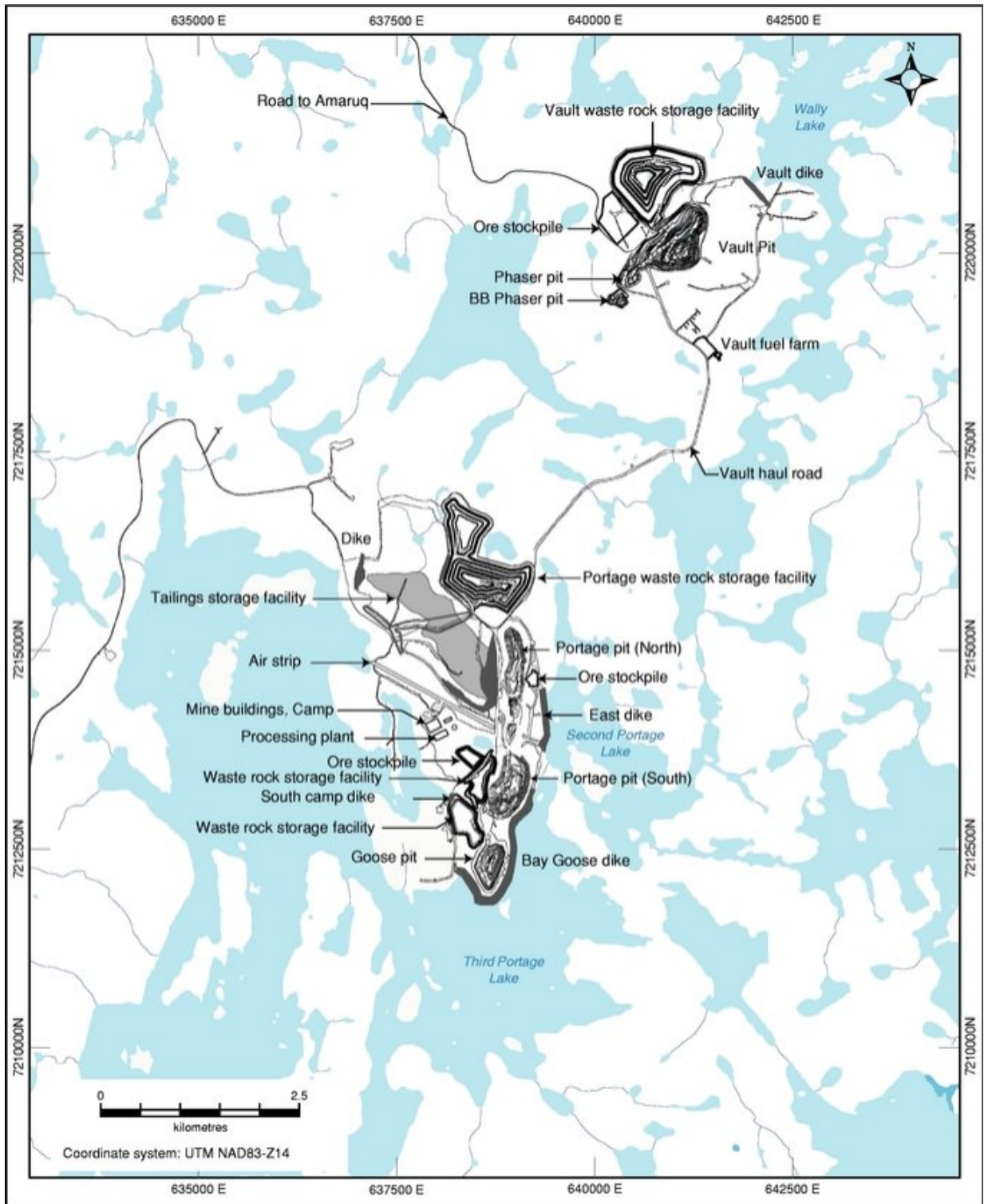
Surface Plan of the Meadowbank Mine (as at December 31, 2017)
