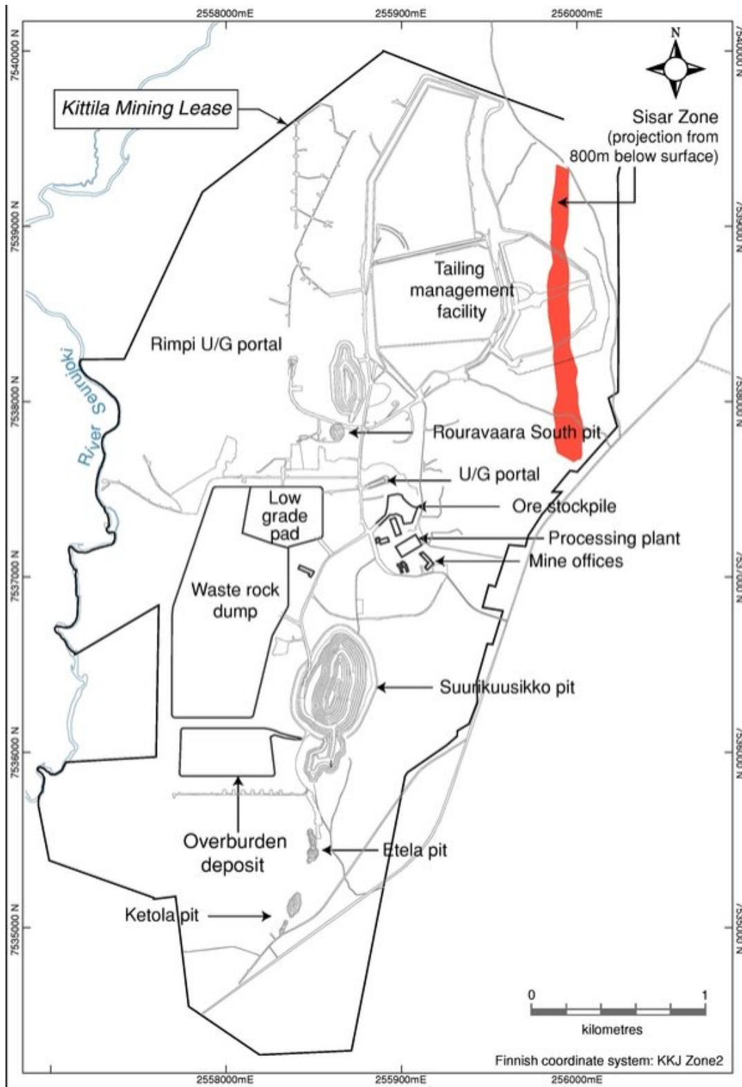
Surface Plan of the Kittila Mine (as at December 31, 2017)
