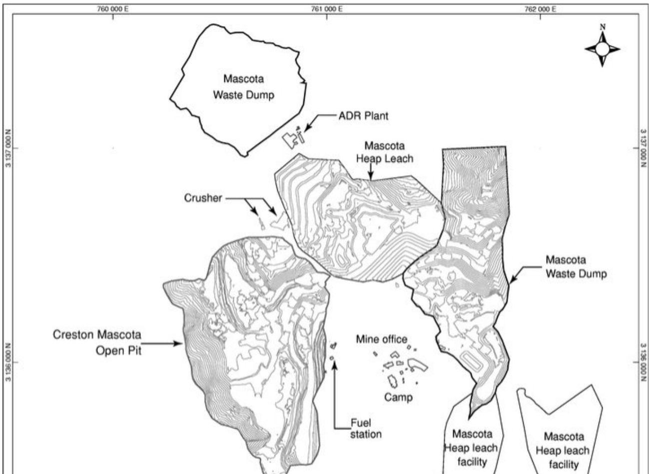
Surface Plan of the Creston Mascota Deposit at Pinos Altos (as at December 31, 2017)
