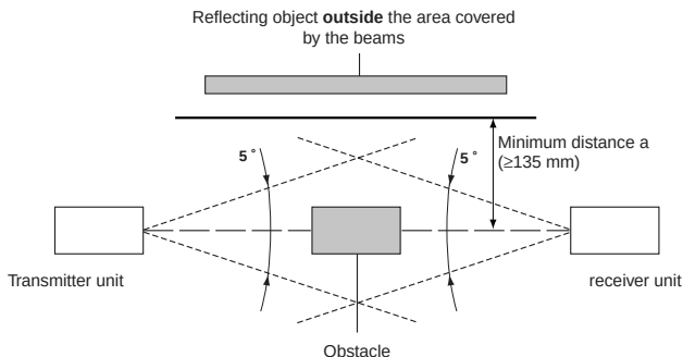
Figure 18.2: Deflection
