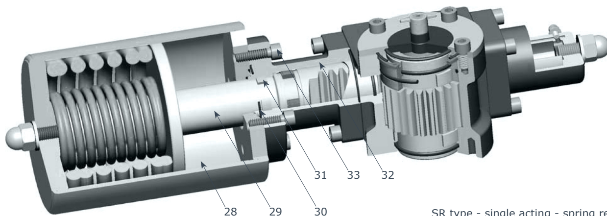
SR type - single acting - spring return
