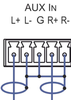
Figure 6: Unbalanced Stereo Audio Input Connection
